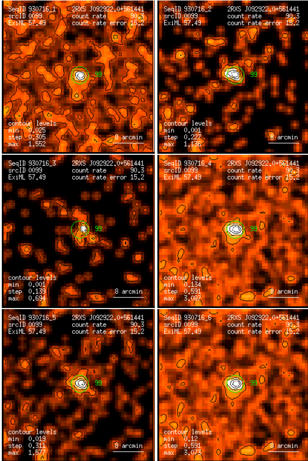
Figure 99: RASS 930716: detection 0099: band rate images, Gaussian filter: (1) PSPC channels 11 – 41, (2) 52 – 90, (3) 91 – 201, (4) 11 – 235, (5) 52 – 201, (6) 11 – 201. Broad band rates in counts/ks. Band rate contour levels in counts/ks/arcmin 2 .
