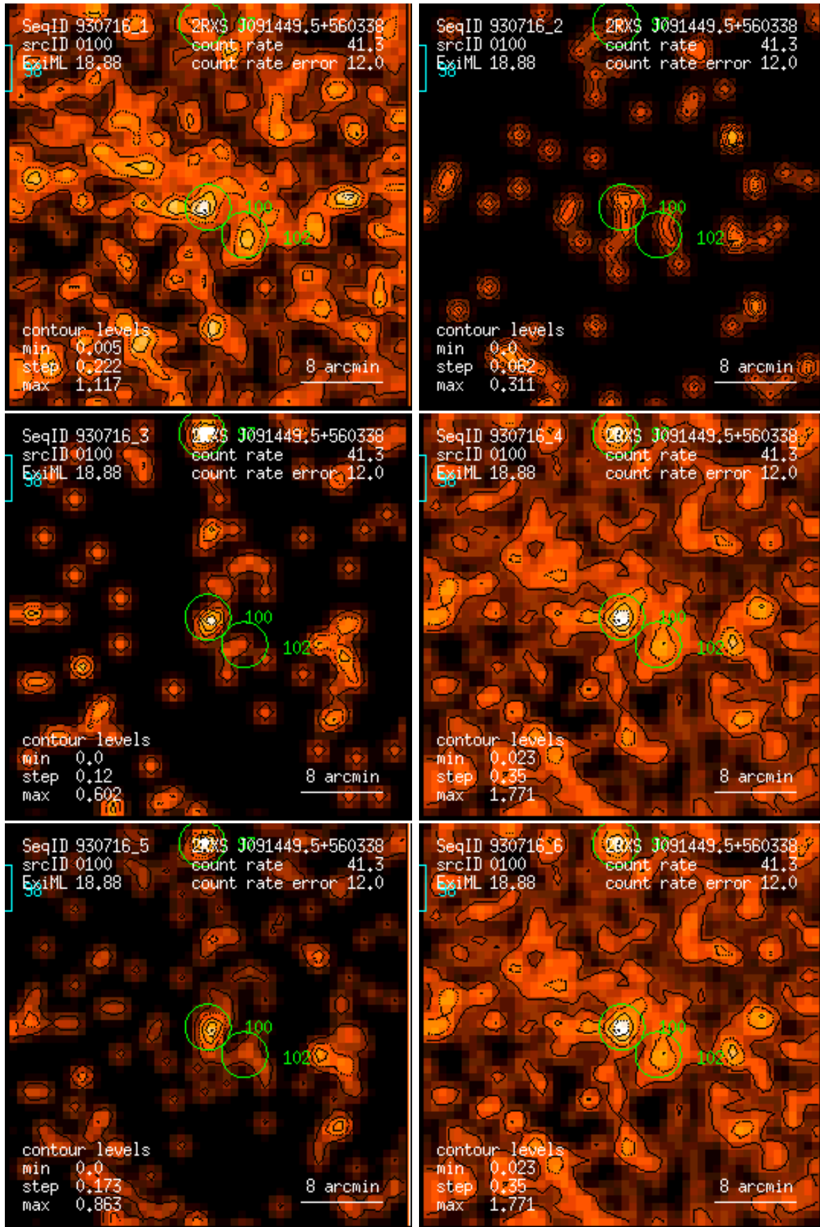
Figure 100: RASS 930716: detection 0100: band rate images, Gaussian filter: (1) PSPC channels 11 – 41, (2) 52 – 90, (3) 91 – 201, (4) 11 – 235, (5) 52 – 201, (6) 11 – 201. Broad band rates in counts/ks. Band rate contour levels in counts/ks/arcmin 2 .
