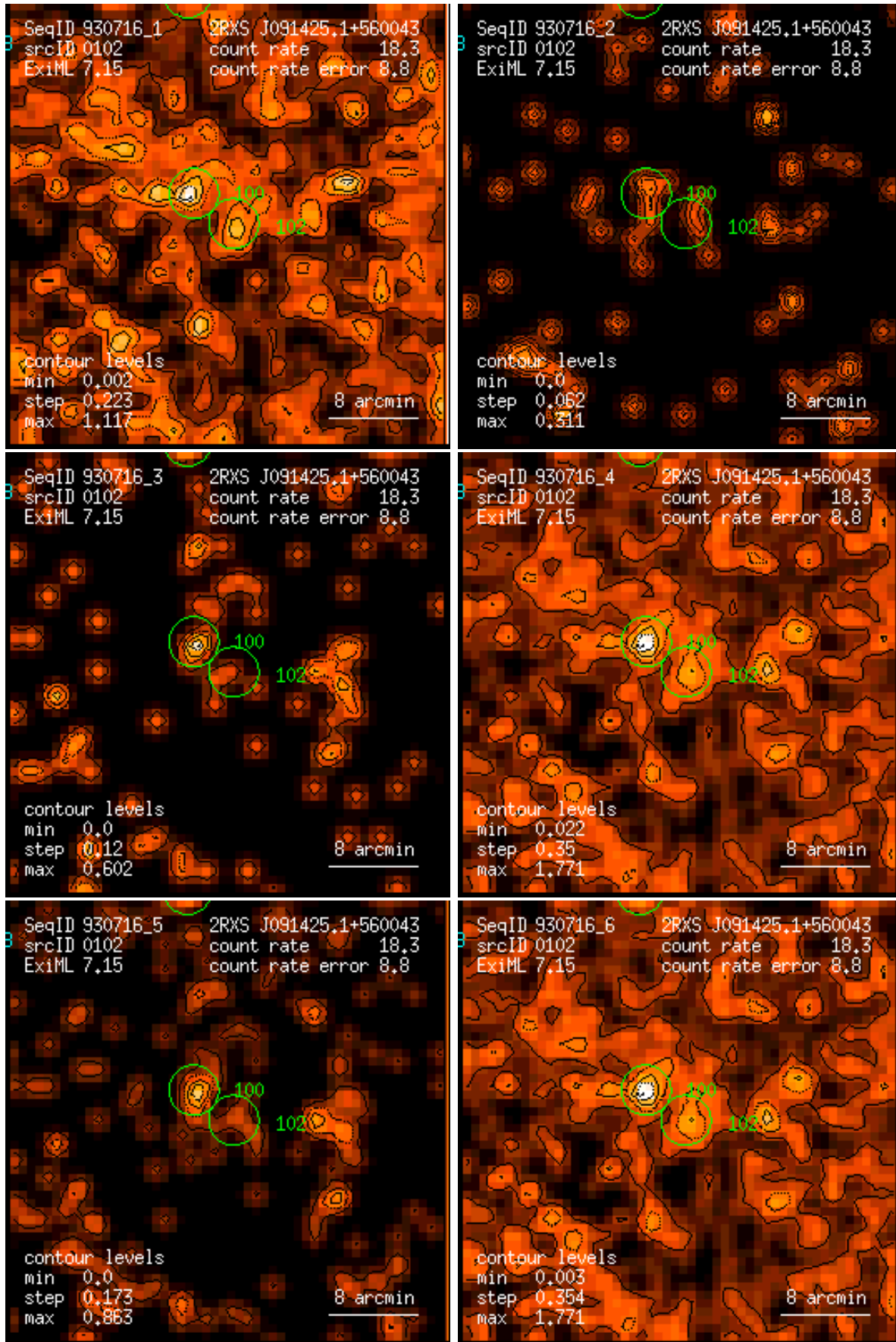
Figure 102: RASS 930716: detection 0102: band rate images, Gaussian filter: (1) PSPC channels 11 – 41, (2) 52 – 90, (3) 91 – 201, (4) 11 – 235, (5) 52 – 201, (6) 11 – 201. Broad band rates in counts/ks. Band rate contour levels in counts/ks/arcmin 2 .
