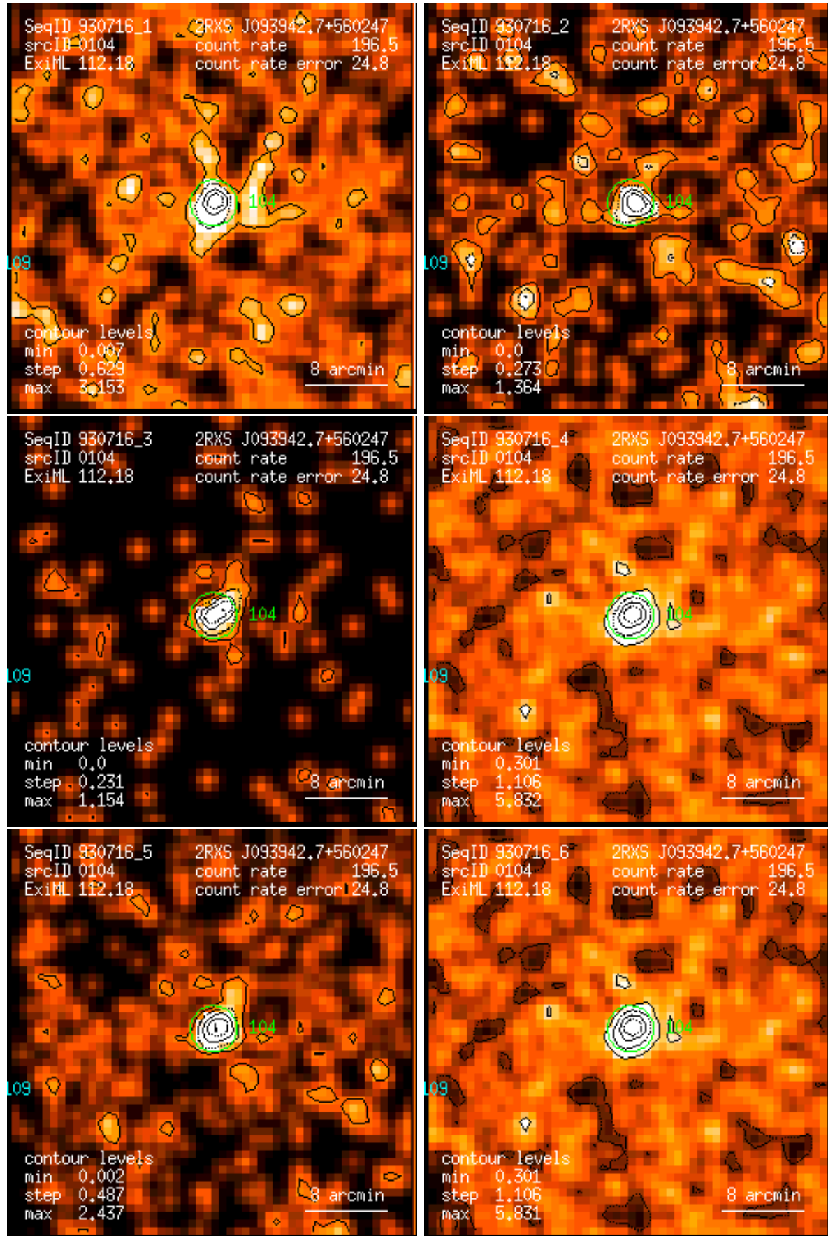
Figure 104: RASS 930716: detection 0104: band rate images, Gaussian filter: (1) PSPC channels 11 – 41, (2) 52 – 90, (3) 91 – 201, (4) 11 – 235, (5) 52 – 201, (6) 11 – 201. Broad band rates in counts/ks. Band rate contour levels in counts/ks/arcmin 2 .
