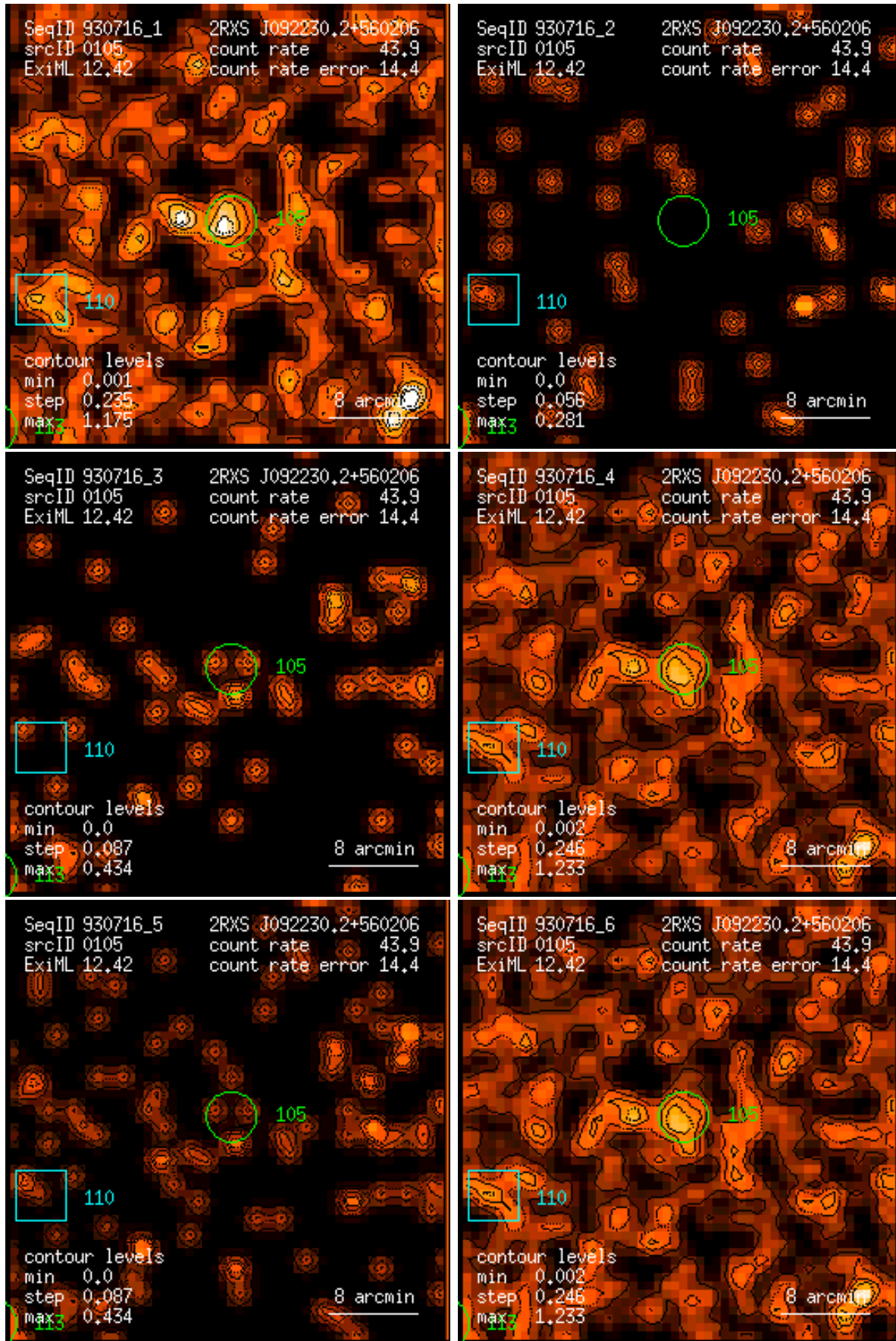
Figure 105: RASS 930716: detection 0105: band rate images, Gaussian filter: (1) PSPC channels 11 – 41, (2) 52 – 90, (3) 91 – 201, (4) 11 – 235, (5) 52 – 201, (6) 11 – 201. Broad band rates in counts/ks. Band rate contour levels in counts/ks/arcmin 2 .
