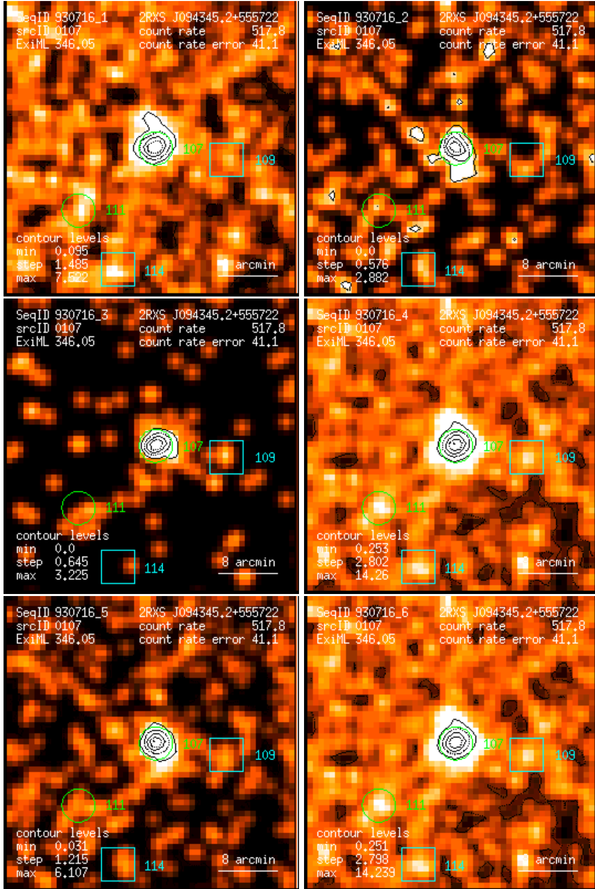
Figure 107: RASS 930716: detection 0107: band rate images, Gaussian filter: (1) PSPC channels 11 – 41, (2) 52 – 90, (3) 91 – 201, (4) 11 – 235, (5) 52 – 201, (6) 11 – 201. Broad band rates in counts/ks. Band rate contour levels in counts/ks/arcmin 2 .
