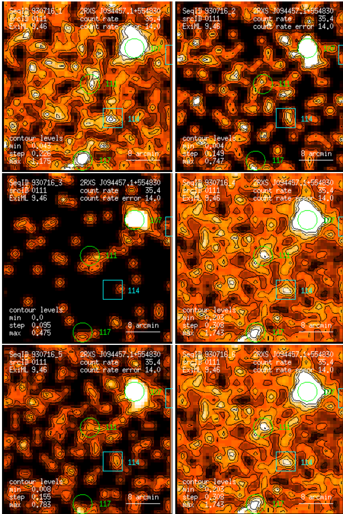
Figure 111: RASS 930716: detection 0111: band rate images, Gaussian filter: (1) PSPC channels 11 – 41, (2) 52 – 90, (3) 91 – 201, (4) 11 – 235, (5) 52 – 201, (6) 11 – 201. Broad band rates in counts/ks. Band rate contour levels in counts/ks/arcmin 2 .
