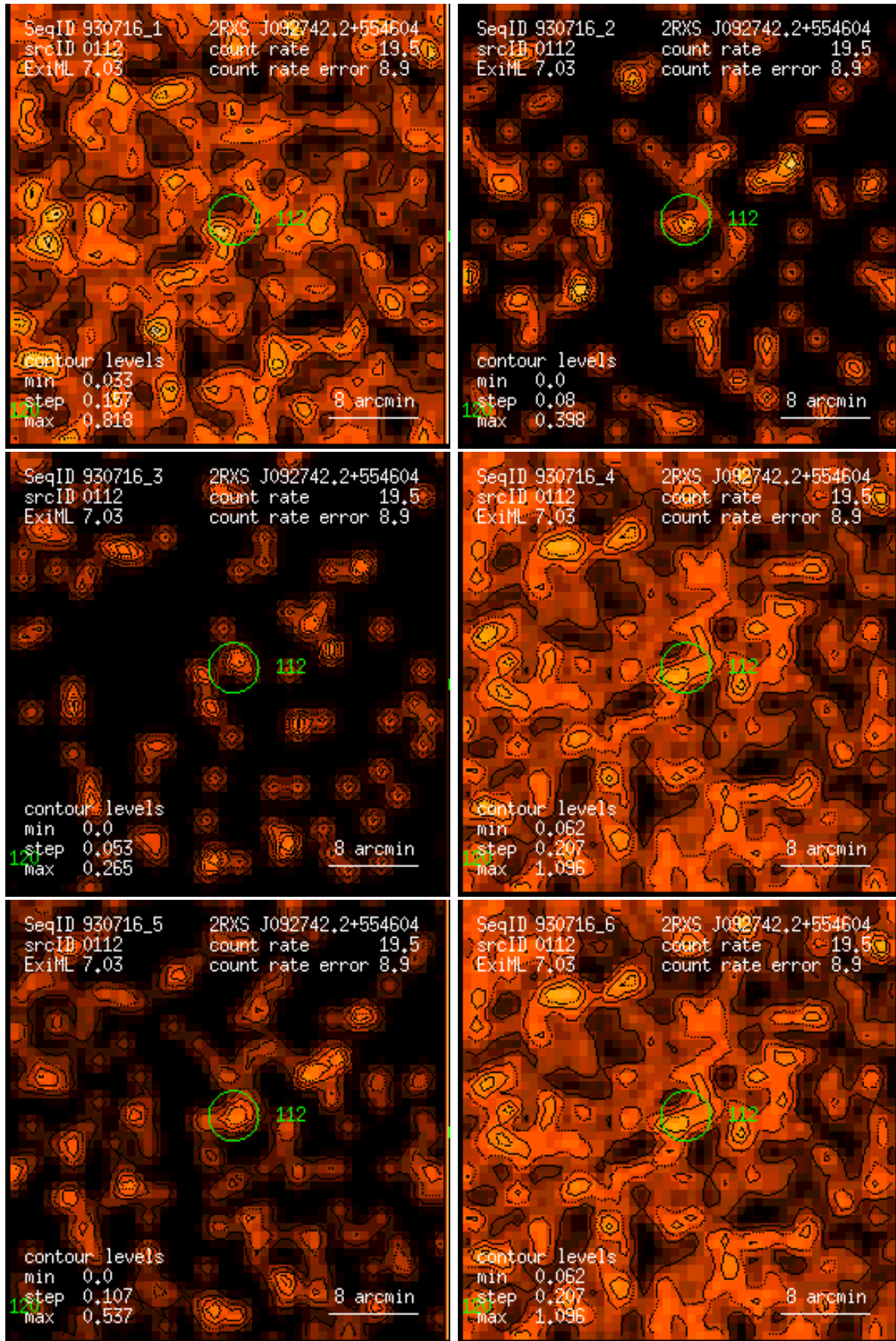
Figure 112: RASS 930716: detection 0112: band rate images, Gaussian filter: (1) PSPC channels 11 – 41, (2) 52 – 90, (3) 91 – 201, (4) 11 – 235, (5) 52 – 201, (6) 11 – 201. Broad band rates in counts/ks. Band rate contour levels in counts/ks/arcmin 2 .
