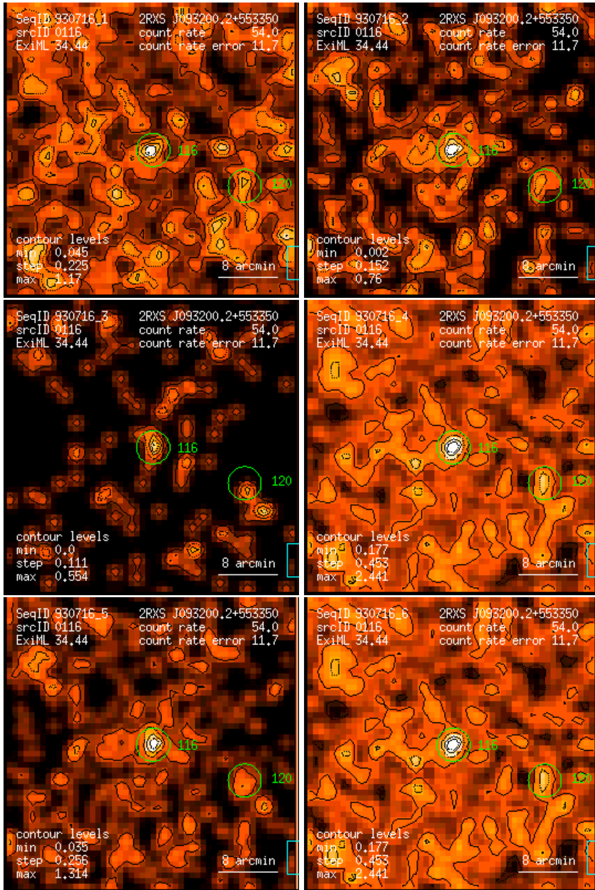
Figure 116: RASS 930716: detection 0116: band rate images, Gaussian filter: (1) PSPC channels 11 – 41, (2) 52 – 90, (3) 91 – 201, (4) 11 – 235, (5) 52 – 201, (6) 11 – 201. Broad band rates in counts/ks. Band rate contour levels in counts/ks/arcmin 2 .
