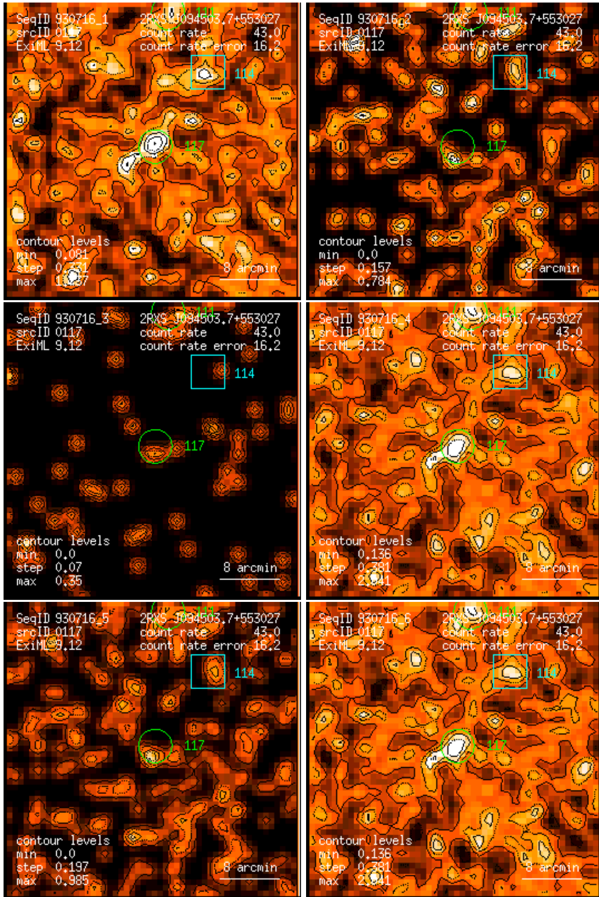
Figure 117: RASS 930716: detection 0117: band rate images, Gaussian filter: (1) PSPC channels 11 – 41, (2) 52 – 90, (3) 91 – 201, (4) 11 – 235, (5) 52 – 201, (6) 11 – 201. Broad band rates in counts/ks. Band rate contour levels in counts/ks/arcmin 2 .
