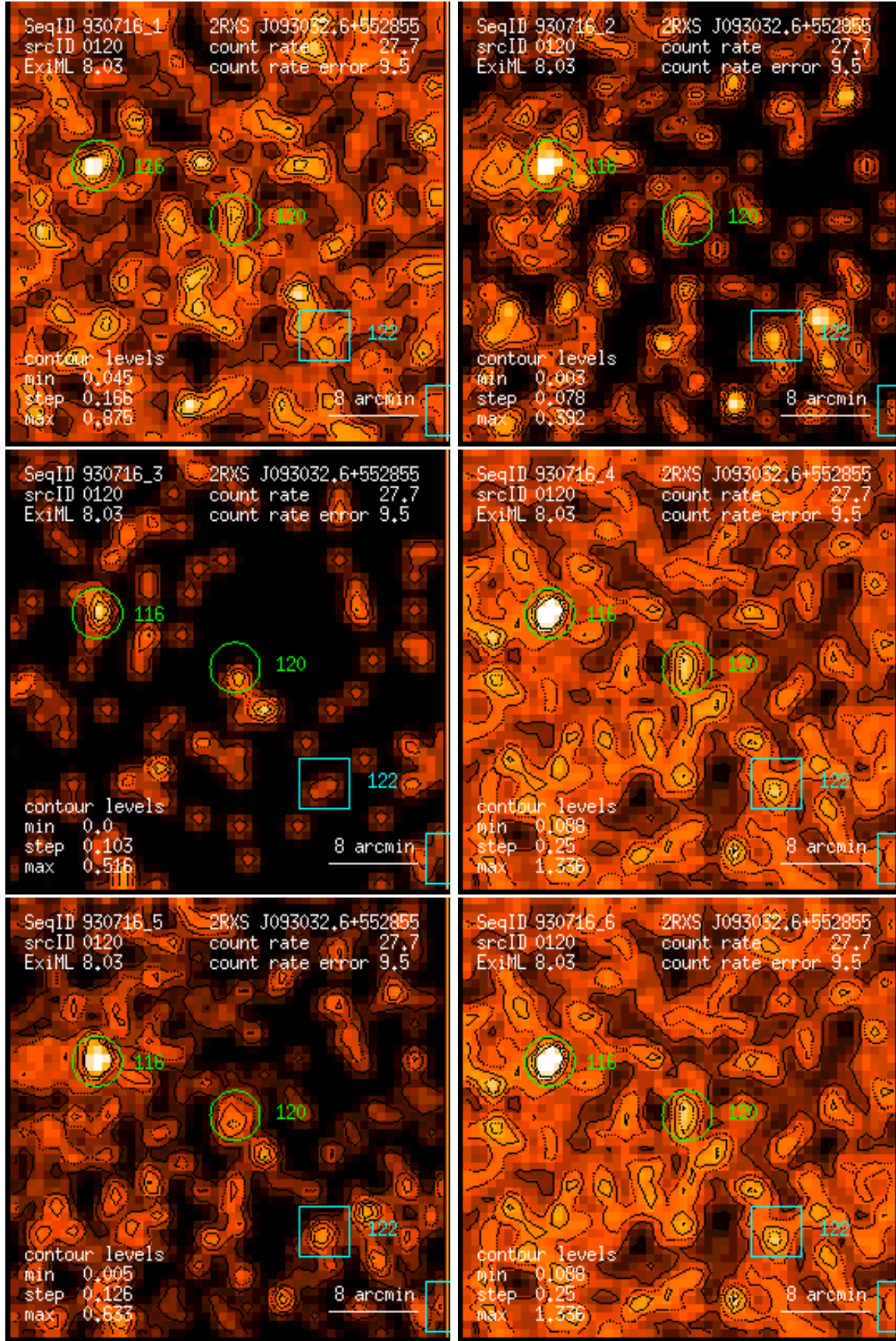
Figure 120: RASS 930716: detection 0120: band rate images, Gaussian filter: (1) PSPC channels 11 – 41, (2) 52 – 90, (3) 91 – 201, (4) 11 – 235, (5) 52 – 201, (6) 11 – 201. Broad band rates in counts/ks. Band rate contour levels in counts/ks/arcmin 2 .
