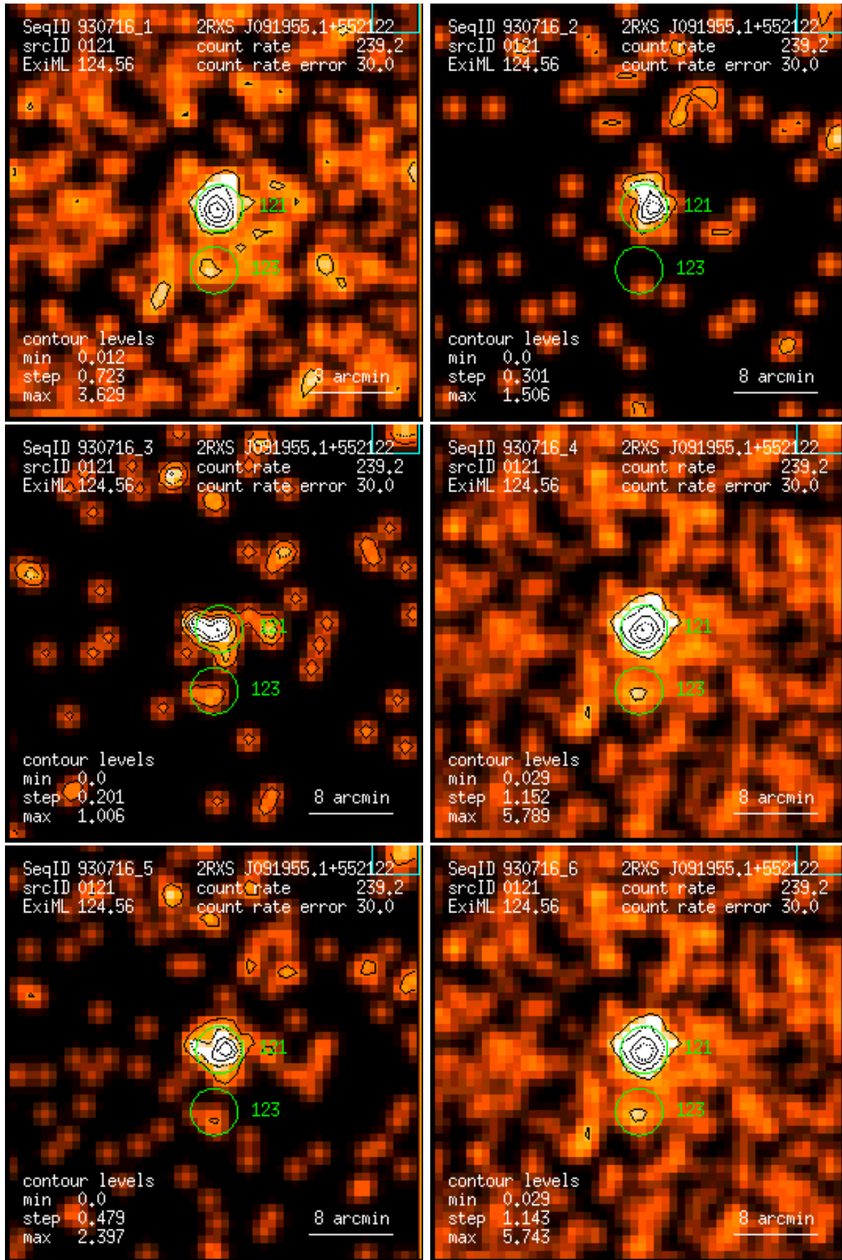
Figure 121: RASS 930716: detection 0121: band rate images, Gaussian filter: (1) PSPC channels 11 – 41, (2) 52 – 90, (3) 91 – 201, (4) 11 – 235, (5) 52 – 201, (6) 11 – 201. Broad band rates in counts/ks. Band rate contour levels in counts/ks/arcmin 2 .
