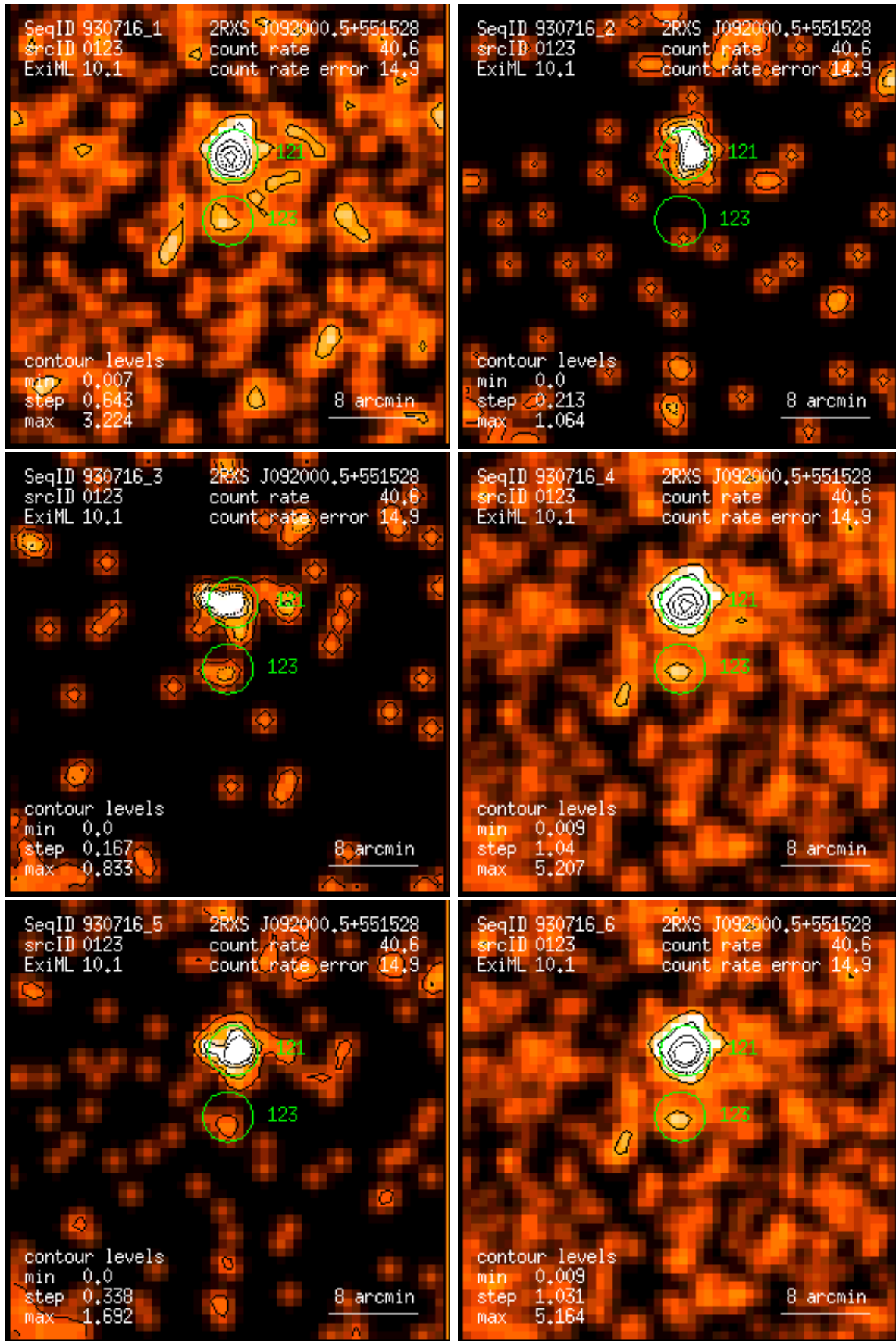
Figure 123: RASS 930716: detection 0123: band rate images, Gaussian filter: (1) PSPC channels 11 – 41, (2) 52 – 90, (3) 91 – 201, (4) 11 – 235, (5) 52 – 201, (6) 11 – 201. Broad band rates in counts/ks. Band rate contour levels in counts/ks/arcmin 2 .
