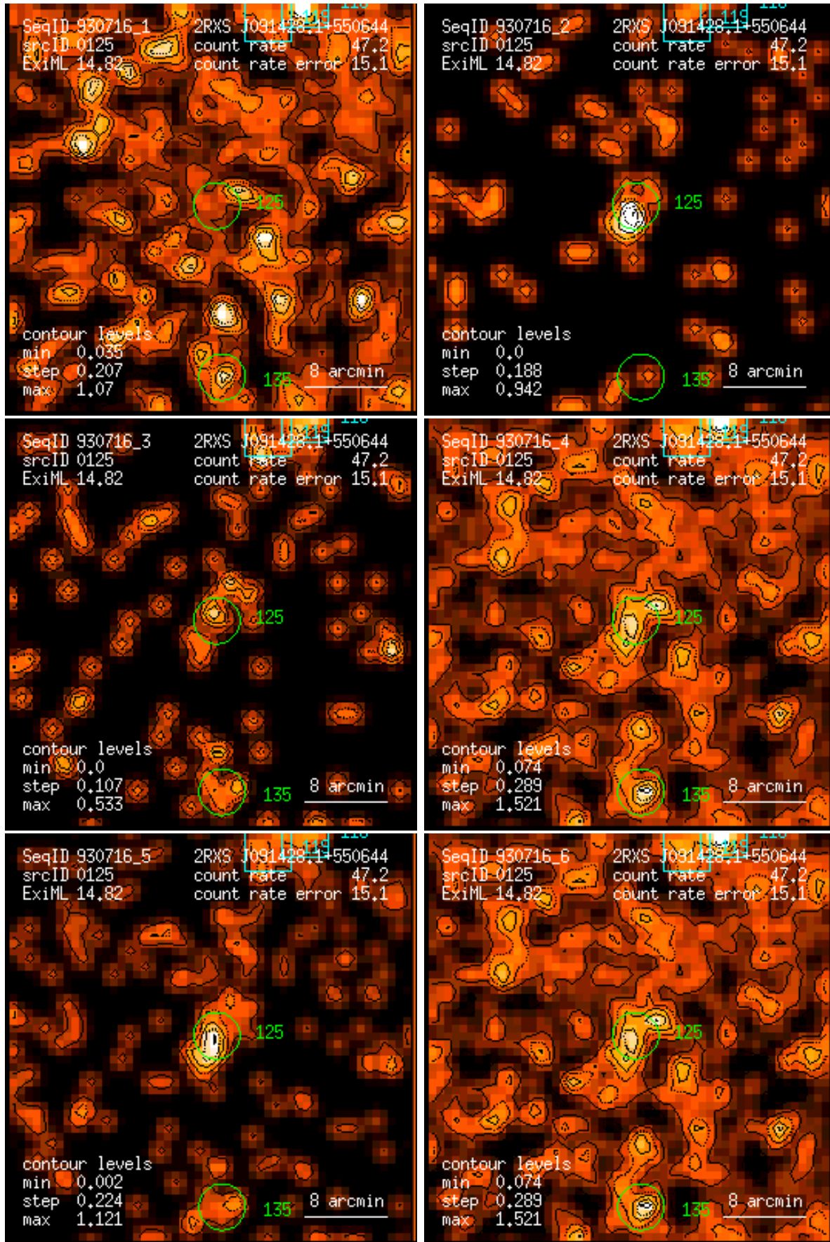
Figure 125: RASS 930716: detection 0125: band rate images, Gaussian filter: (1) PSPC channels 11 – 41, (2) 52 – 90, (3) 91 – 201, (4) 11 – 235, (5) 52 – 201, (6) 11 – 201. Broad band rates in counts/ks. Band rate contour levels in counts/ks/arcmin 2 .
