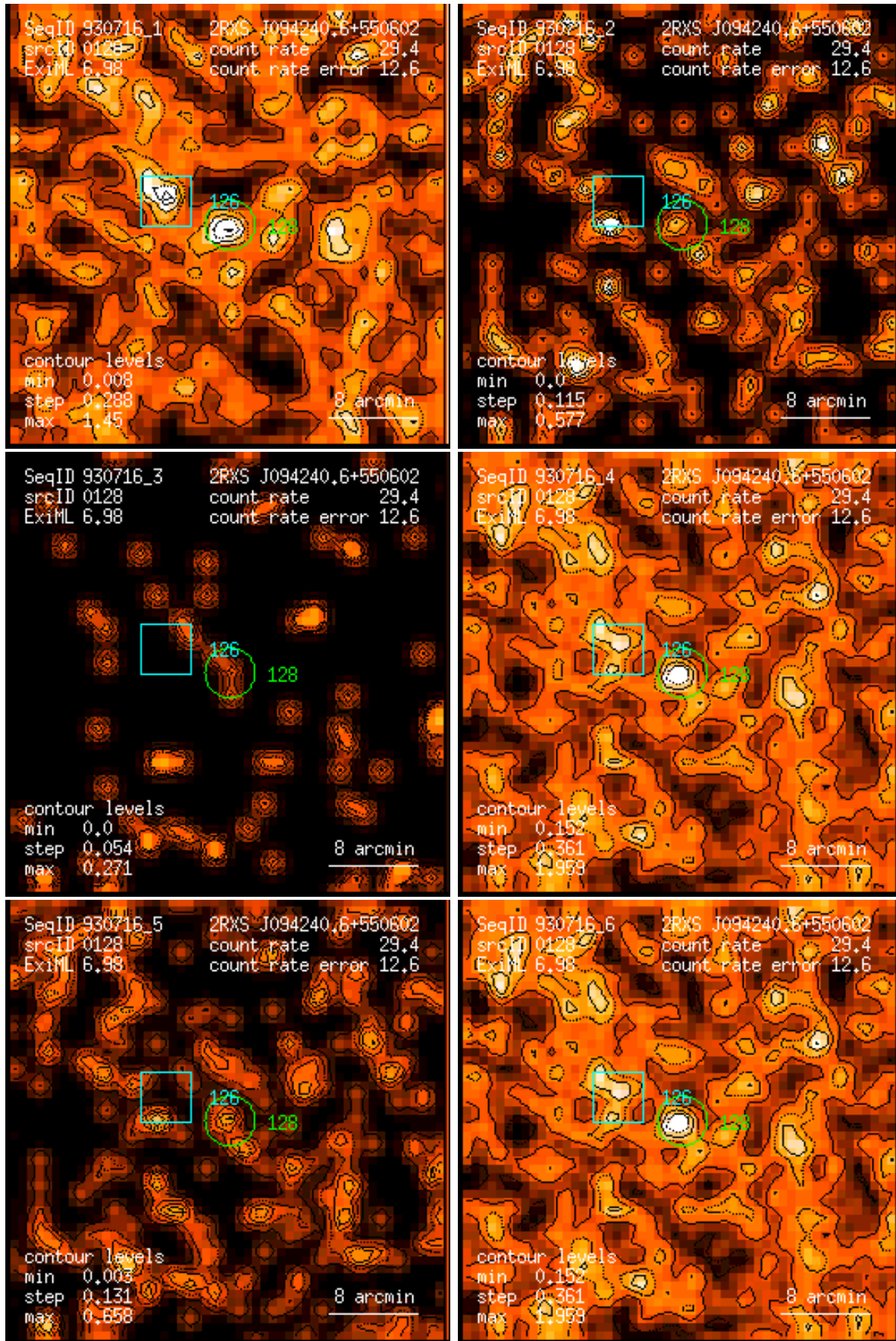
Figure 128: RASS 930716: detection 0128: band rate images, Gaussian filter: (1) PSPC channels 11 – 41, (2) 52 – 90, (3) 91 – 201, (4) 11 – 235, (5) 52 – 201, (6) 11 – 201. Broad band rates in counts/ks. Band rate contour levels in counts/ks/arcmin 2 .
