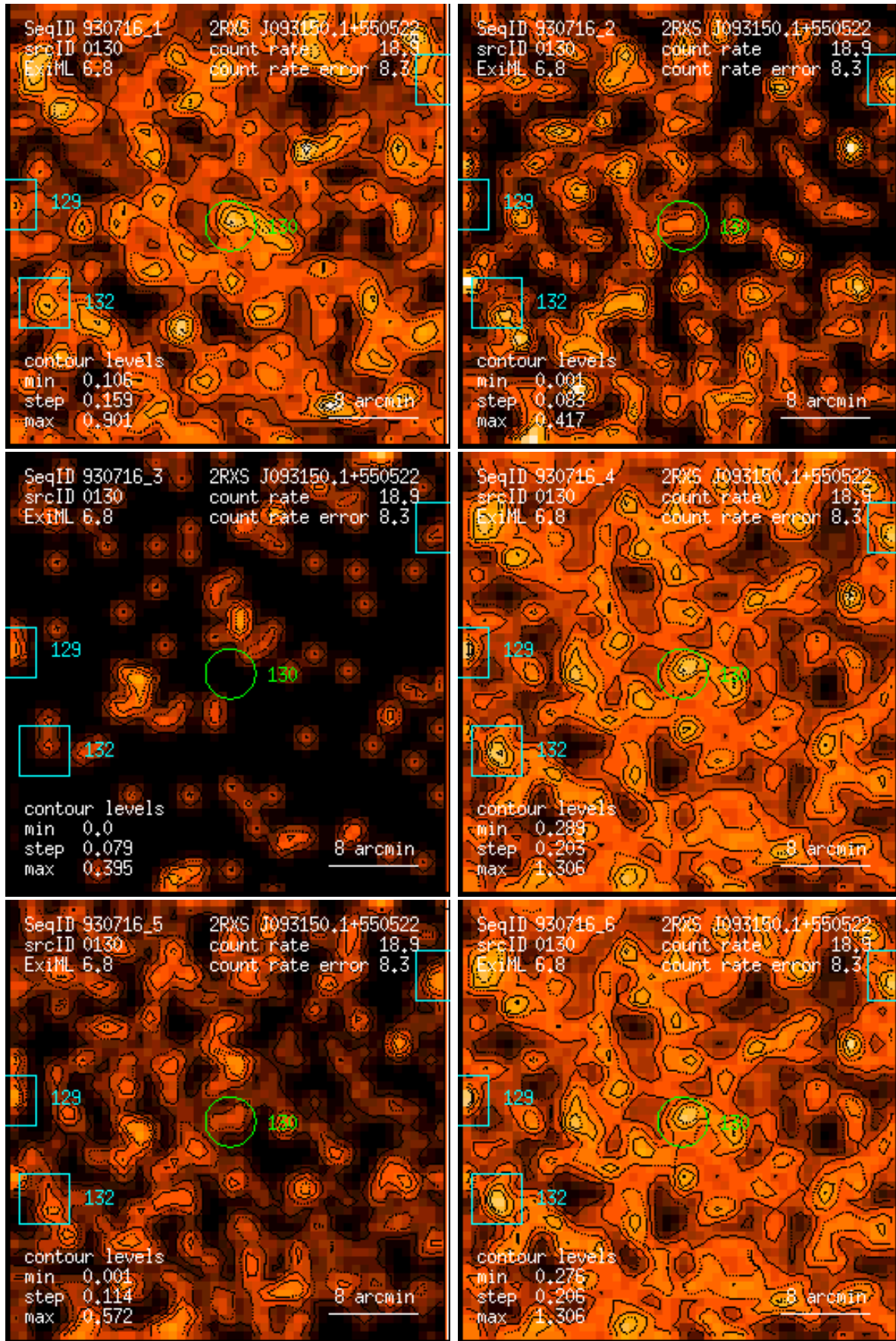
Figure 130: RASS 930716: detection 0130: band rate images, Gaussian filter: (1) PSPC channels 11 – 41, (2) 52 – 90, (3) 91 – 201, (4) 11 – 235, (5) 52 – 201, (6) 11 – 201. Broad band rates in counts/ks. Band rate contour levels in counts/ks/arcmin 2 .
