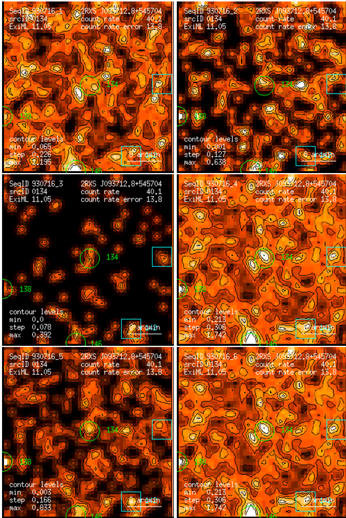
Figure 134: RASS 930716: detection 0134: band rate images, Gaussian filter: (1) PSPC channels 11 – 41, (2) 52 – 90, (3) 91 – 201, (4) 11 – 235, (5) 52 – 201, (6) 11 – 201. Broad band rates in counts/ks. Band rate contour levels in counts/ks/arcmin 2 .
