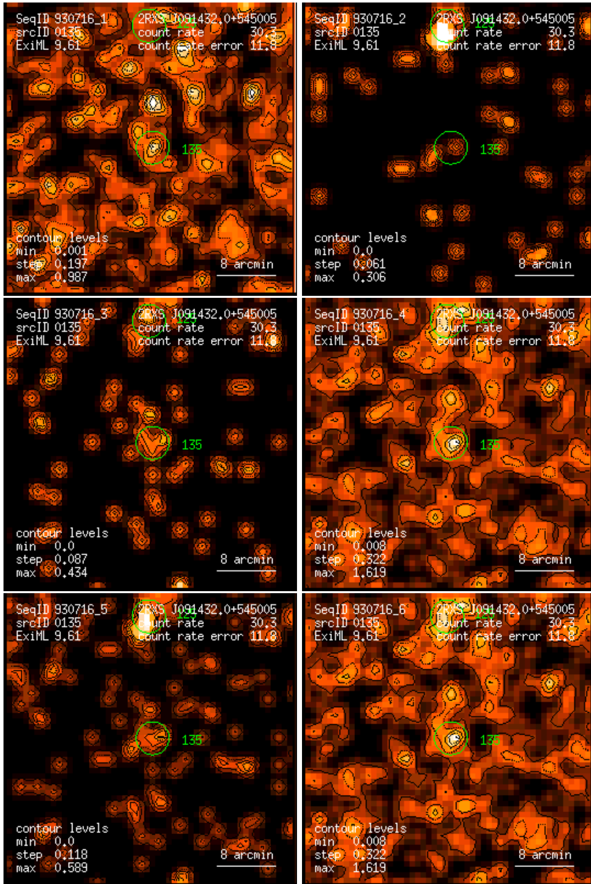
Figure 135: RASS 930716: detection 0135: band rate images, Gaussian filter: (1) PSPC channels 11 – 41, (2) 52 – 90, (3) 91 – 201, (4) 11 – 235, (5) 52 – 201, (6) 11 – 201. Broad band rates in counts/ks. Band rate contour levels in counts/ks/arcmin 2 .
