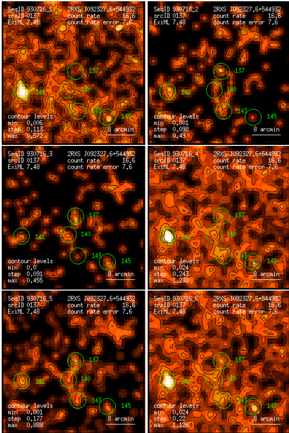
Figure 137: RASS 930716: detection 0137: band rate images, Gaussian filter: (1) PSPC channels 11 – 41, (2) 52 – 90, (3) 91 – 201, (4) 11 – 235, (5) 52 – 201, (6) 11 – 201. Broad band rates in counts/ks. Band rate contour levels in counts/ks/arcmin 2 .
