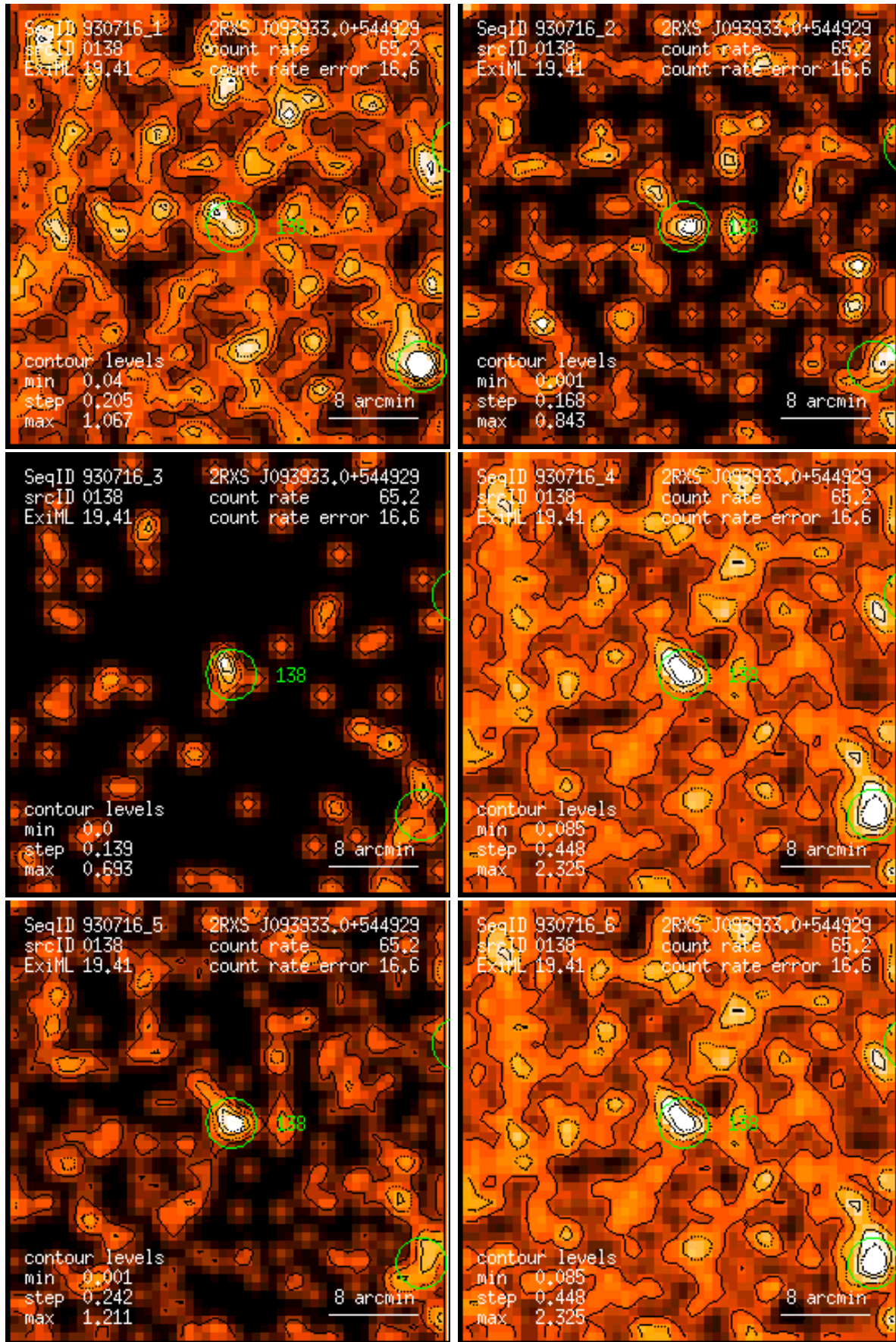
Figure 138: RASS 930716: detection 0138: band rate images, Gaussian filter: (1) PSPC channels 11 – 41, (2) 52 – 90, (3) 91 – 201, (4) 11 – 235, (5) 52 – 201, (6) 11 – 201. Broad band rates in counts/ks. Band rate contour levels in counts/ks/arcmin 2 .
