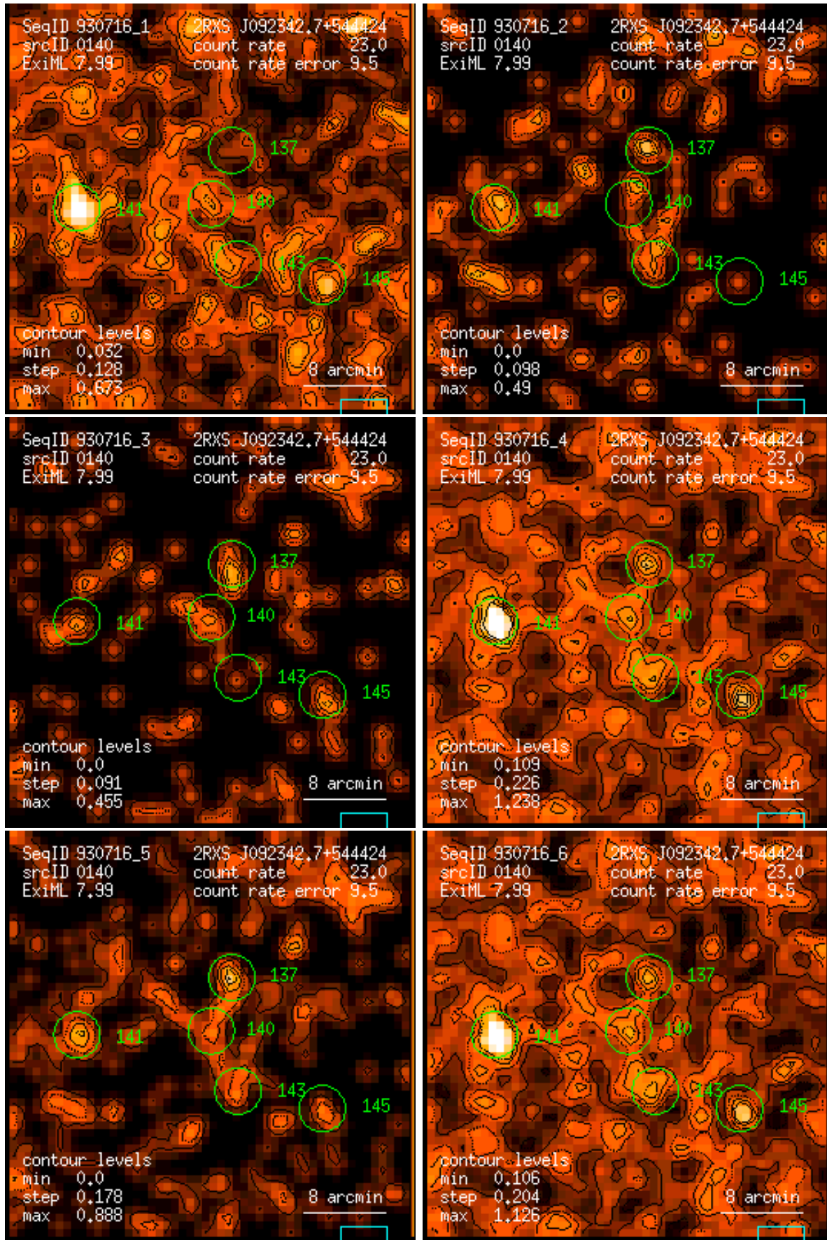
Figure 140: RASS 930716: detection 0140: band rate images, Gaussian filter: (1) PSPC channels 11 – 41, (2) 52 – 90, (3) 91 – 201, (4) 11 – 235, (5) 52 – 201, (6) 11 – 201. Broad band rates in counts/ks. Band rate contour levels in counts/ks/arcmin 2 .
