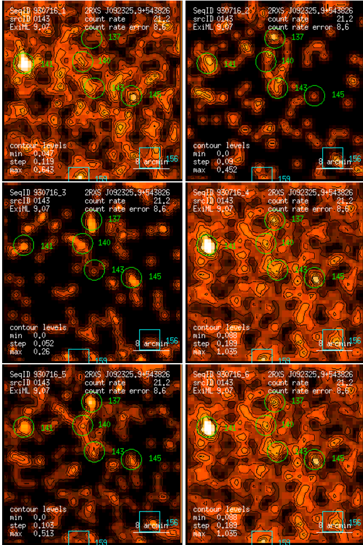
Figure 143: RASS 930716: detection 0143: band rate images, Gaussian filter: (1) PSPC channels 11 – 41, (2) 52 – 90, (3) 91 – 201, (4) 11 – 235, (5) 52 – 201, (6) 11 – 201. Broad band rates in counts/ks. Band rate contour levels in counts/ks/arcmin 2 .
