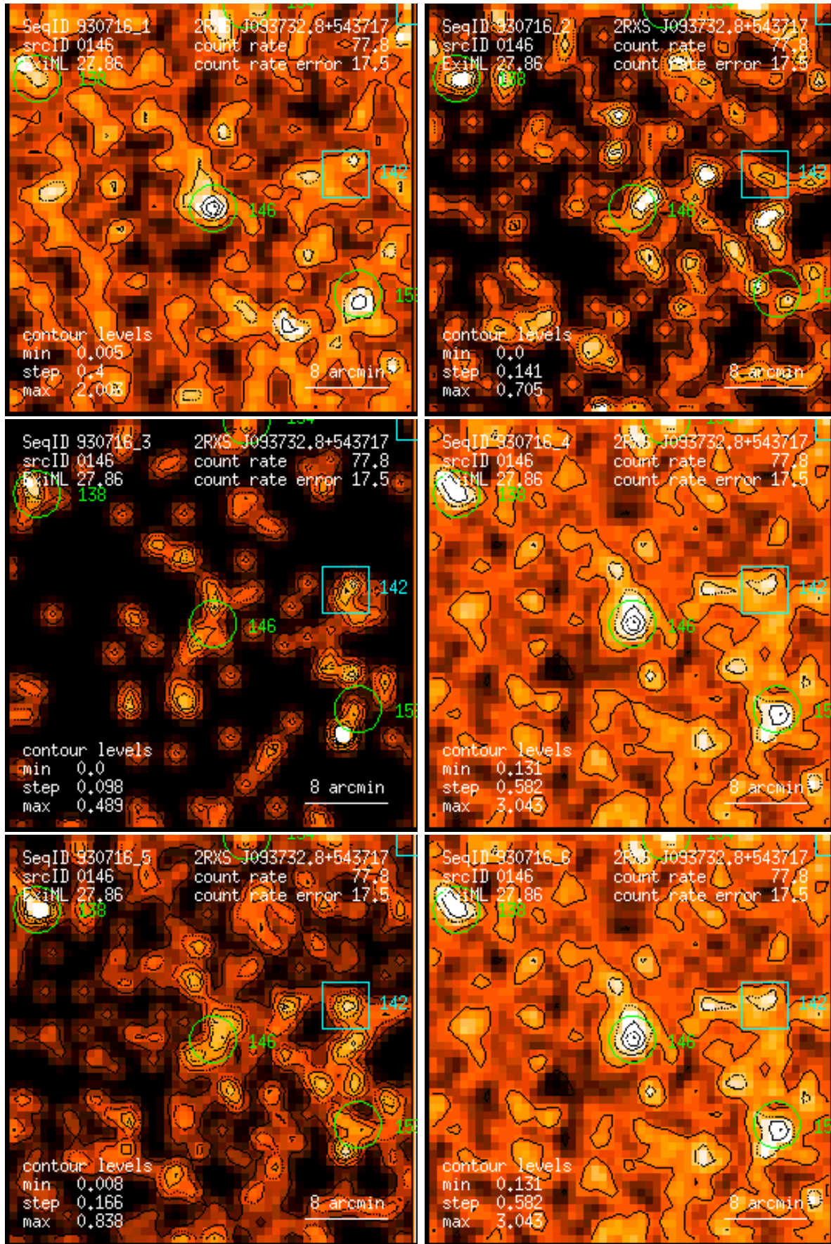
Figure 146: RASS 930716: detection 0146: band rate images, Gaussian filter: (1) PSPC channels 11 – 41, (2) 52 – 90, (3) 91 – 201, (4) 11 – 235, (5) 52 – 201, (6) 11 – 201. Broad band rates in counts/ks. Band rate contour levels in counts/ks/arcmin 2 .
