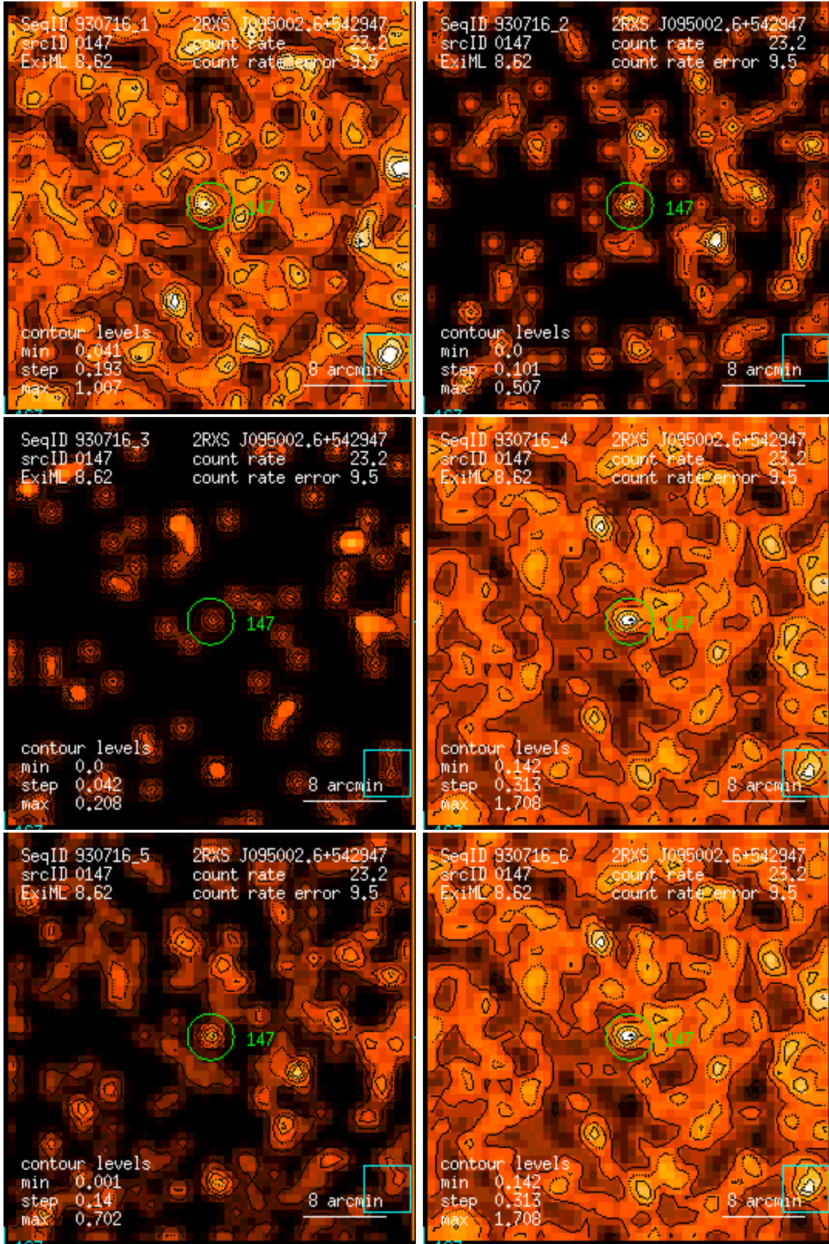
Figure 147: RASS 930716: detection 0147: band rate images, Gaussian filter: (1) PSPC channels 11 – 41, (2) 52 – 90, (3) 91 – 201, (4) 11 – 235, (5) 52 – 201, (6) 11 – 201. Broad band rates in counts/ks. Band rate contour levels in counts/ks/arcmin 2 .
