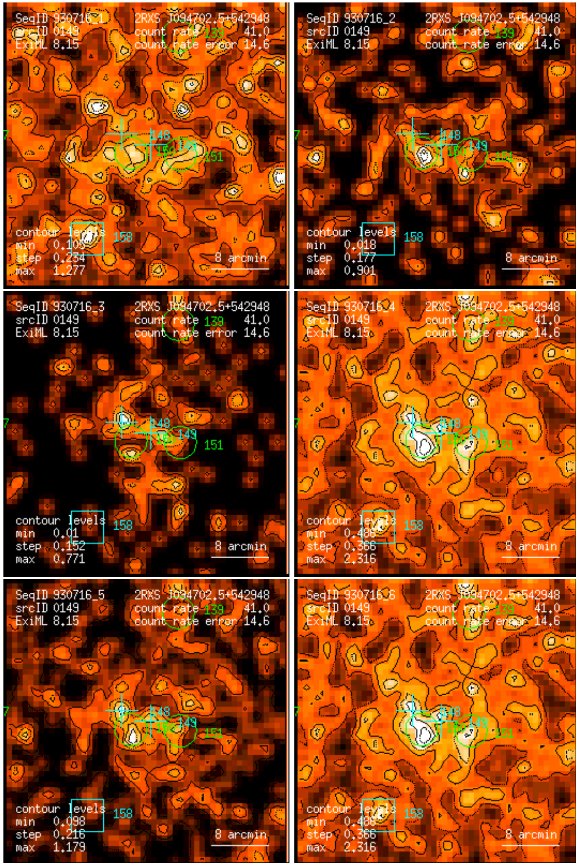
Figure 149: RASS 930716: detection 0149: band rate images, Gaussian filter: (1) PSPC channels 11 – 41, (2) 52 – 90, (3) 91 – 201, (4) 11 – 235, (5) 52 – 201, (6) 11 – 201. Broad band rates in counts/ks. Band rate contour levels in counts/ks/arcmin 2 .
