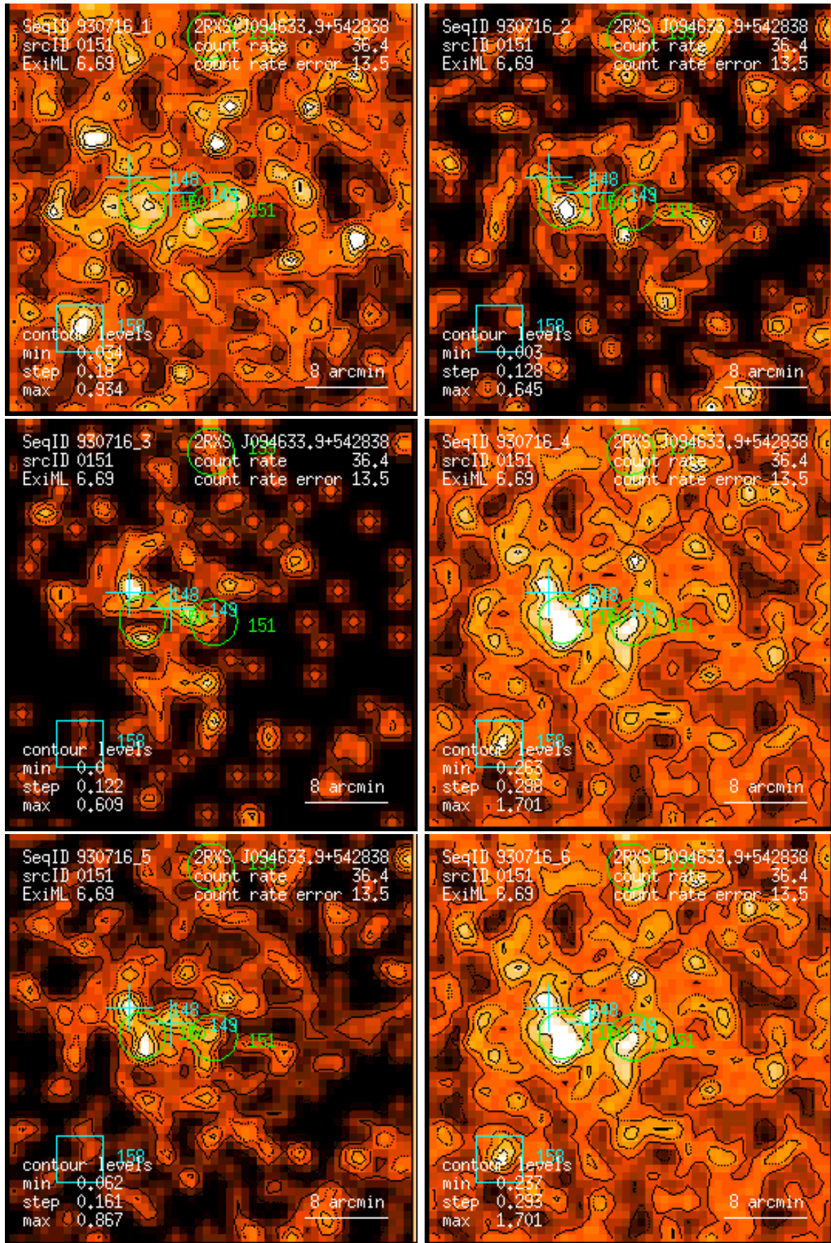
Figure 151: RASS 930716: detection 0151: band rate images, Gaussian filter: (1) PSPC channels 11 – 41, (2) 52 – 90, (3) 91 – 201, (4) 11 – 235, (5) 52 – 201, (6) 11 – 201. Broad band rates in counts/ks. Band rate contour levels in counts/ks/arcmin 2 .
