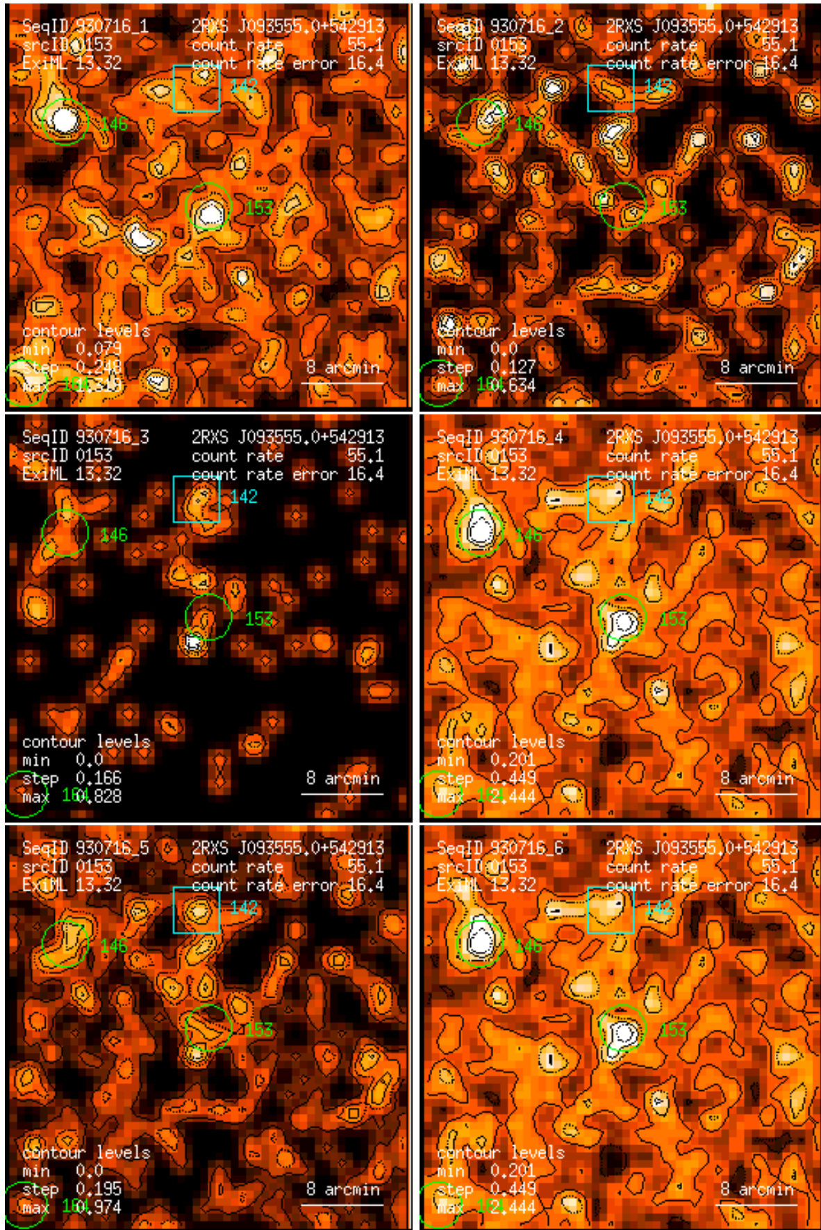
Figure 153: RASS 930716: detection 0153: band rate images, Gaussian filter: (1) PSPC channels 11 – 41, (2) 52 – 90, (3) 91 – 201, (4) 11 – 235, (5) 52 – 201, (6) 11 – 201. Broad band rates in counts/ks. Band rate contour levels in counts/ks/arcmin 2 .
