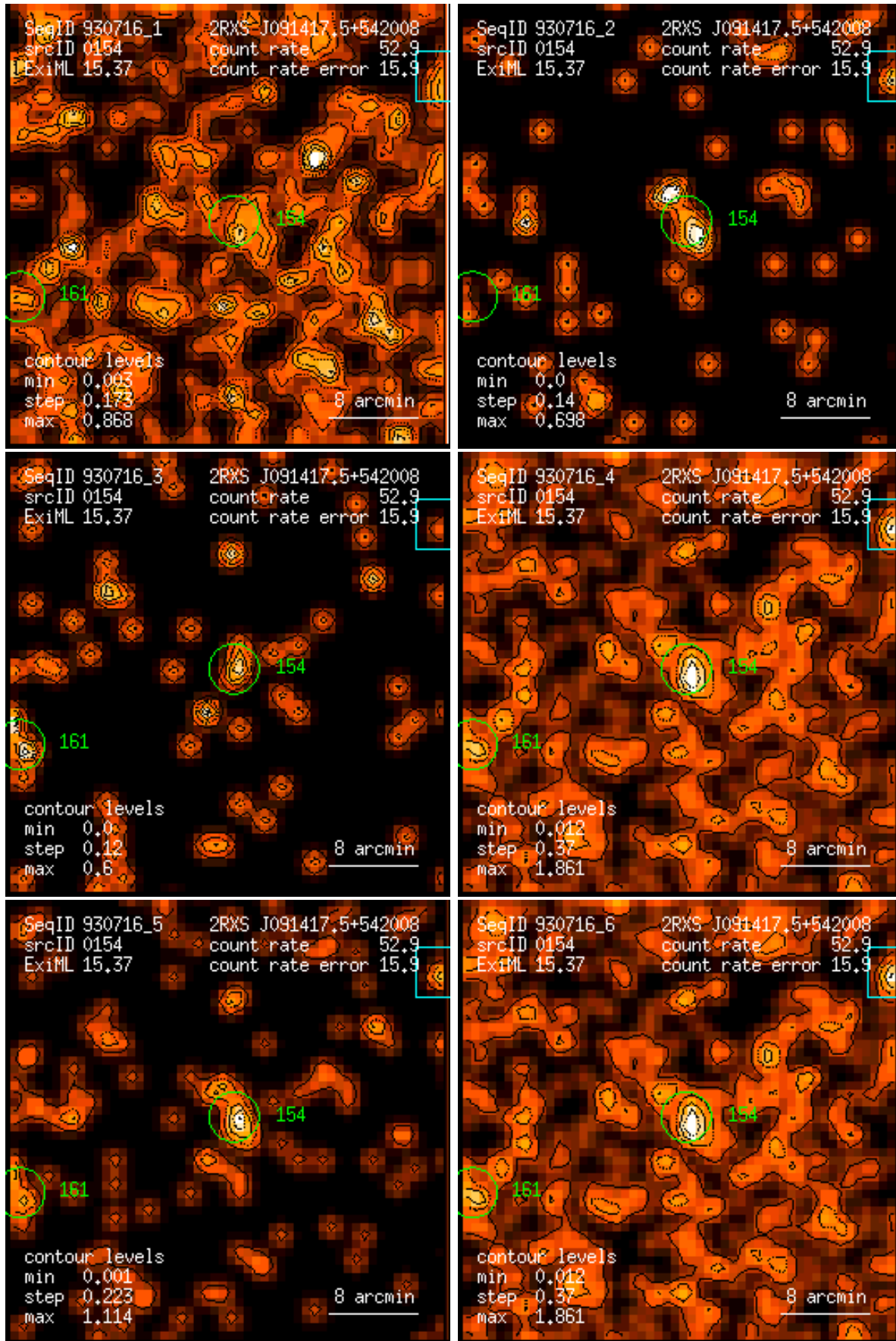
Figure 154: RASS 930716: detection 0154: band rate images, Gaussian filter: (1) PSPC channels 11 – 41, (2) 52 – 90, (3) 91 – 201, (4) 11 – 235, (5) 52 – 201, (6) 11 – 201. Broad band rates in counts/ks. Band rate contour levels in counts/ks/arcmin 2 .
