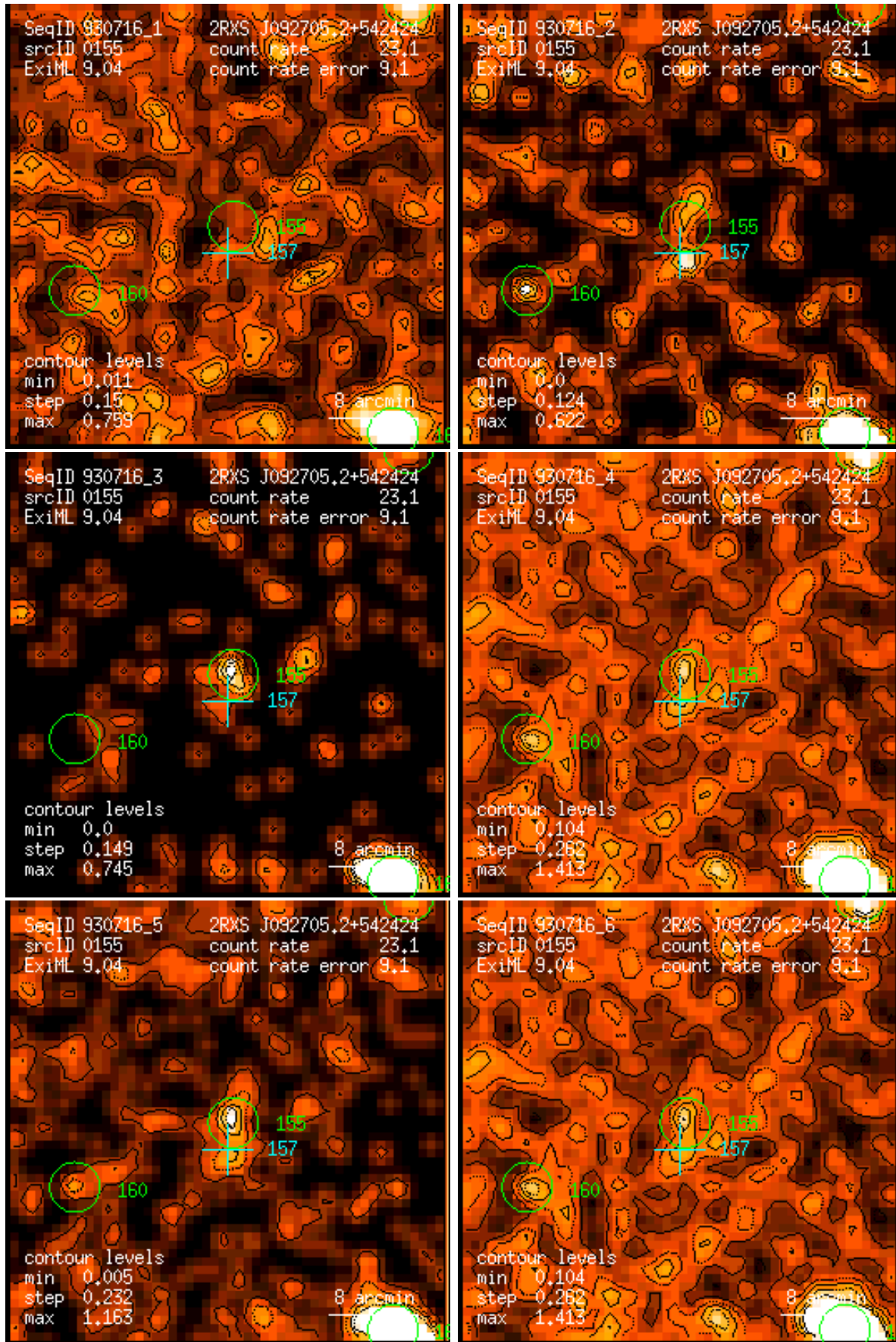
Figure 155: RASS 930716: detection 0155: band rate images, Gaussian filter: (1) PSPC channels 11 – 41, (2) 52 – 90, (3) 91 – 201, (4) 11 – 235, (5) 52 – 201, (6) 11 – 201. Broad band rates in counts/ks. Band rate contour levels in counts/ks/arcmin 2 .
