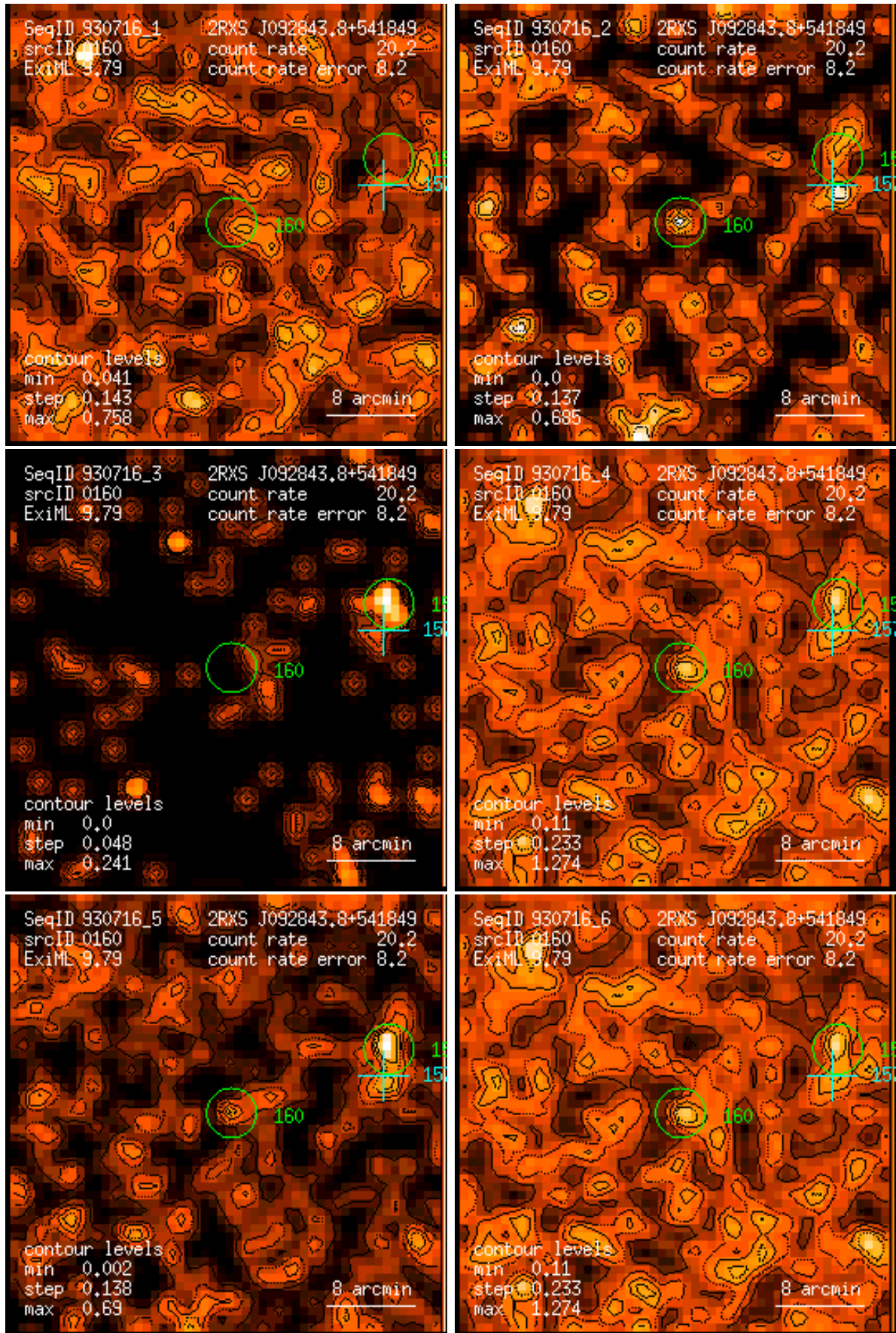
Figure 160: RASS 930716: detection 0160: band rate images, Gaussian filter: (1) PSPC channels 11 – 41, (2) 52 – 90, (3) 91 – 201, (4) 11 – 235, (5) 52 – 201, (6) 11 – 201. Broad band rates in counts/ks. Band rate contour levels in counts/ks/arcmin 2 .
