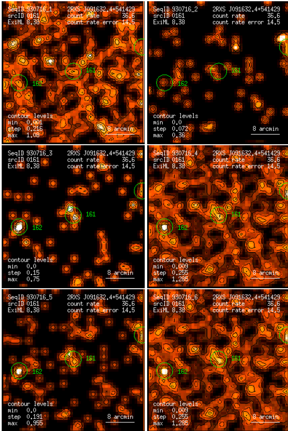
Figure 161: RASS 930716: detection 0161: band rate images, Gaussian filter: (1) PSPC channels 11 – 41, (2) 52 – 90, (3) 91 – 201, (4) 11 – 235, (5) 52 – 201, (6) 11 – 201. Broad band rates in counts/ks. Band rate contour levels in counts/ks/arcmin 2 .
