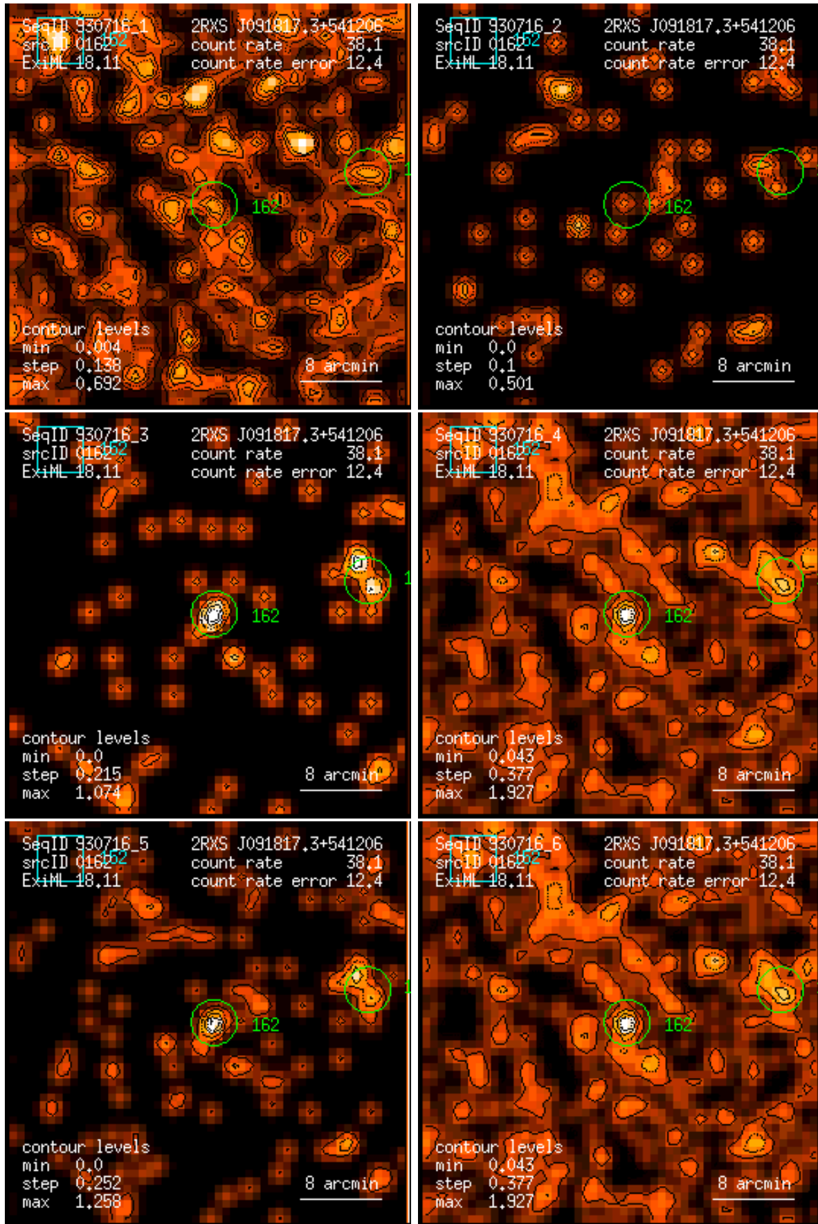
Figure 162: RASS 930716: detection 0162: band rate images, Gaussian filter: (1) PSPC channels 11 – 41, (2) 52 – 90, (3) 91 – 201, (4) 11 – 235, (5) 52 – 201, (6) 11 – 201. Broad band rates in counts/ks. Band rate contour levels in counts/ks/arcmin 2 .
