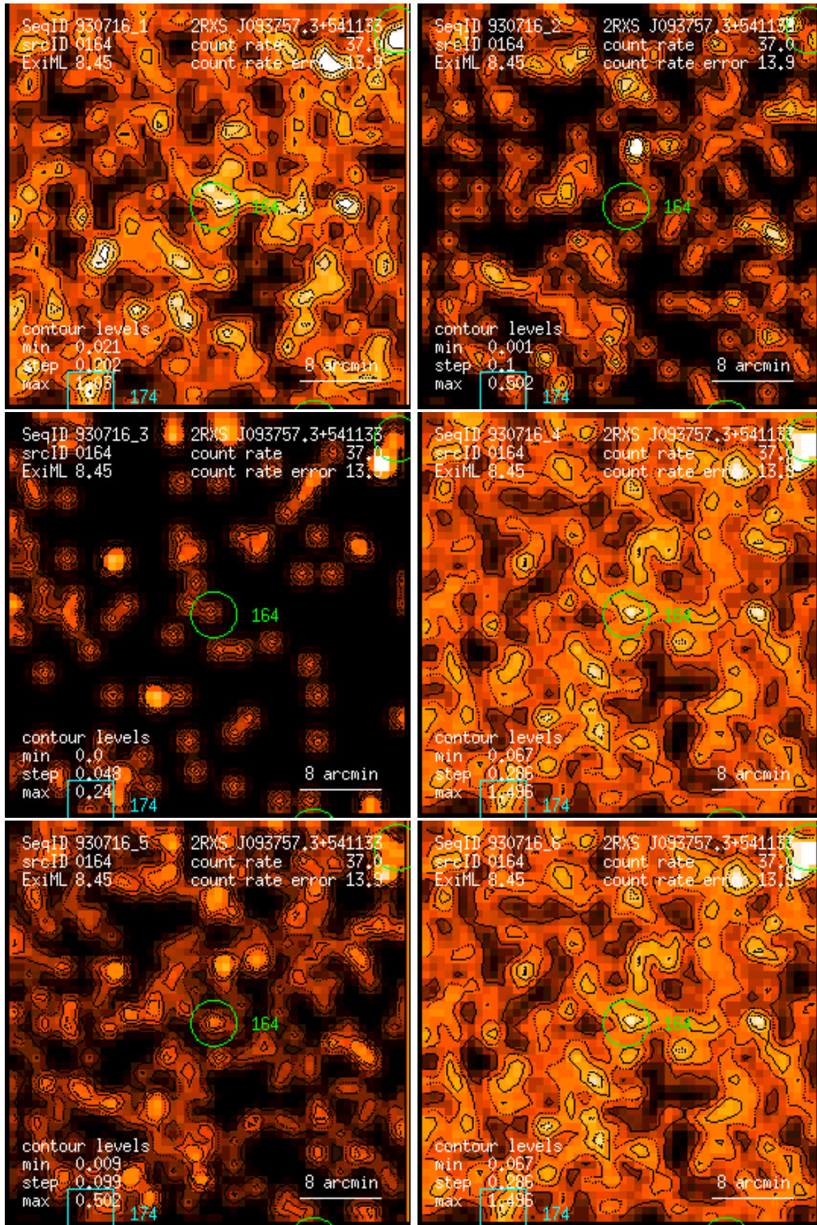
Figure 164: RASS 930716: detection 0164: band rate images, Gaussian filter: (1) PSPC channels 11 – 41, (2) 52 – 90, (3) 91 – 201, (4) 11 – 235, (5) 52 – 201, (6) 11 – 201. Broad band rates in counts/ks. Band rate contour levels in counts/ks/arcmin 2 .
