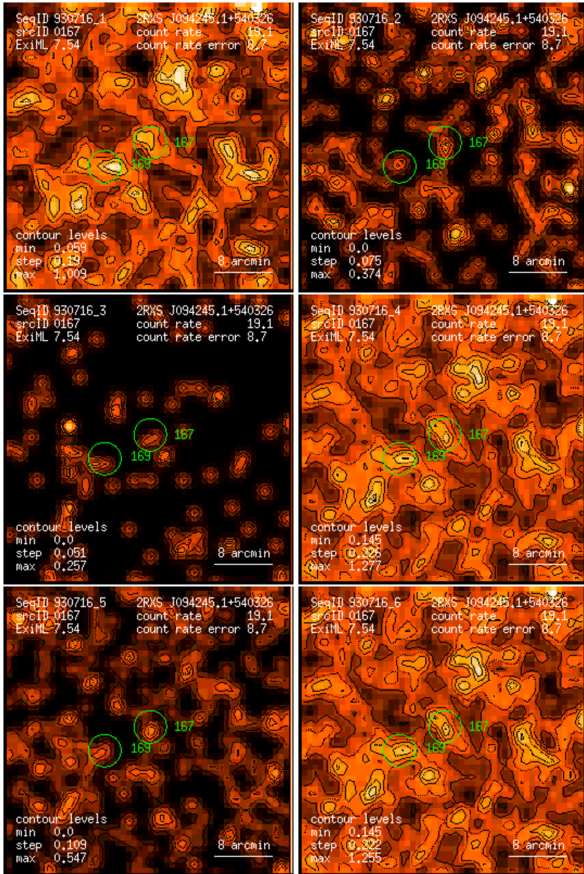
Figure 167: RASS 930716: detection 0167: band rate images, Gaussian filter: (1) PSPC channels 11 – 41, (2) 52 – 90, (3) 91 – 201, (4) 11 – 235, (5) 52 – 201, (6) 11 – 201. Broad band rates in counts/ks. Band rate contour levels in counts/ks/arcmin 2 .
