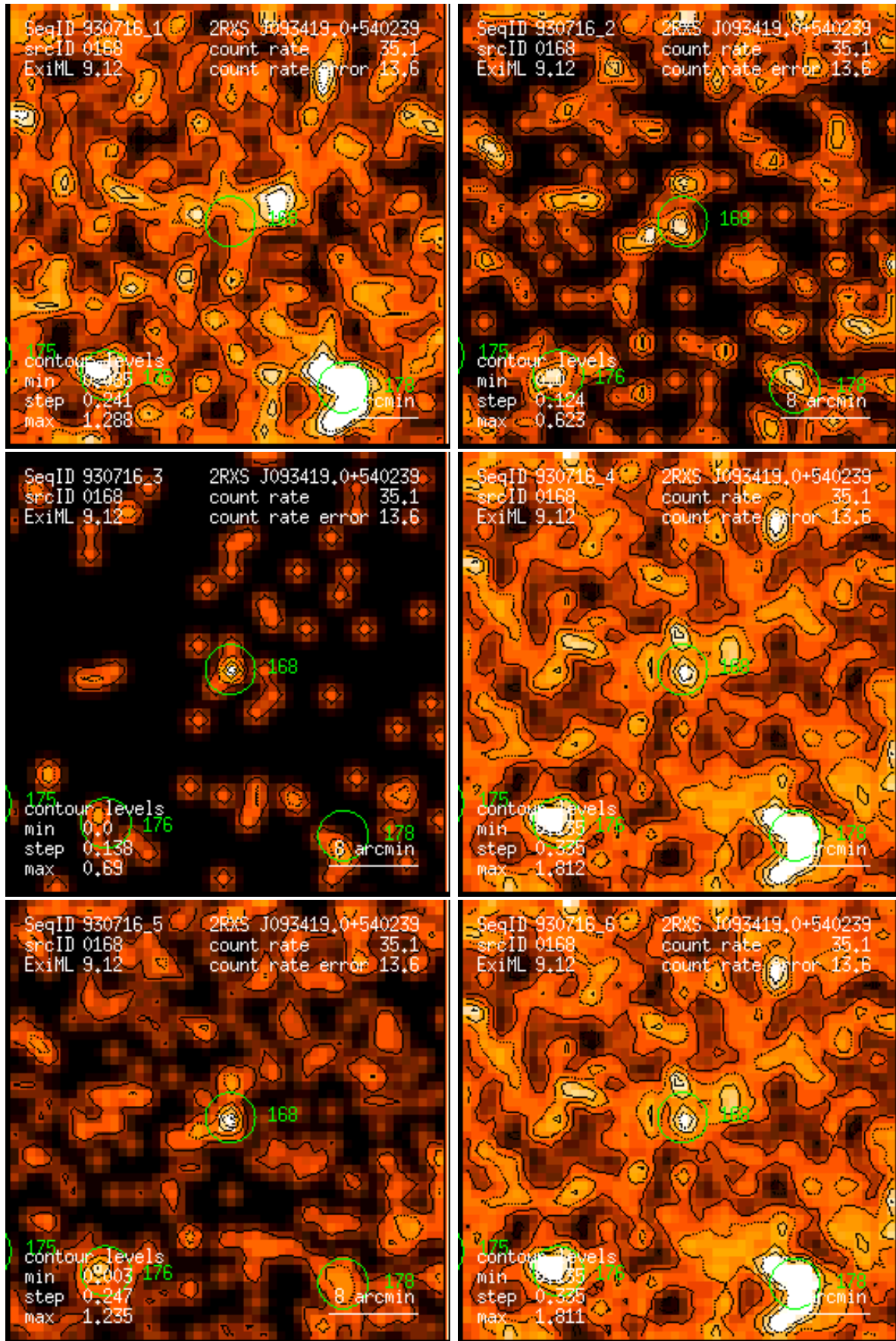
Figure 168: RASS 930716: detection 0168: band rate images, Gaussian filter: (1) PSPC channels 11 – 41, (2) 52 – 90, (3) 91 – 201, (4) 11 – 235, (5) 52 – 201, (6) 11 – 201. Broad band rates in counts/ks. Band rate contour levels in counts/ks/arcmin 2 .
