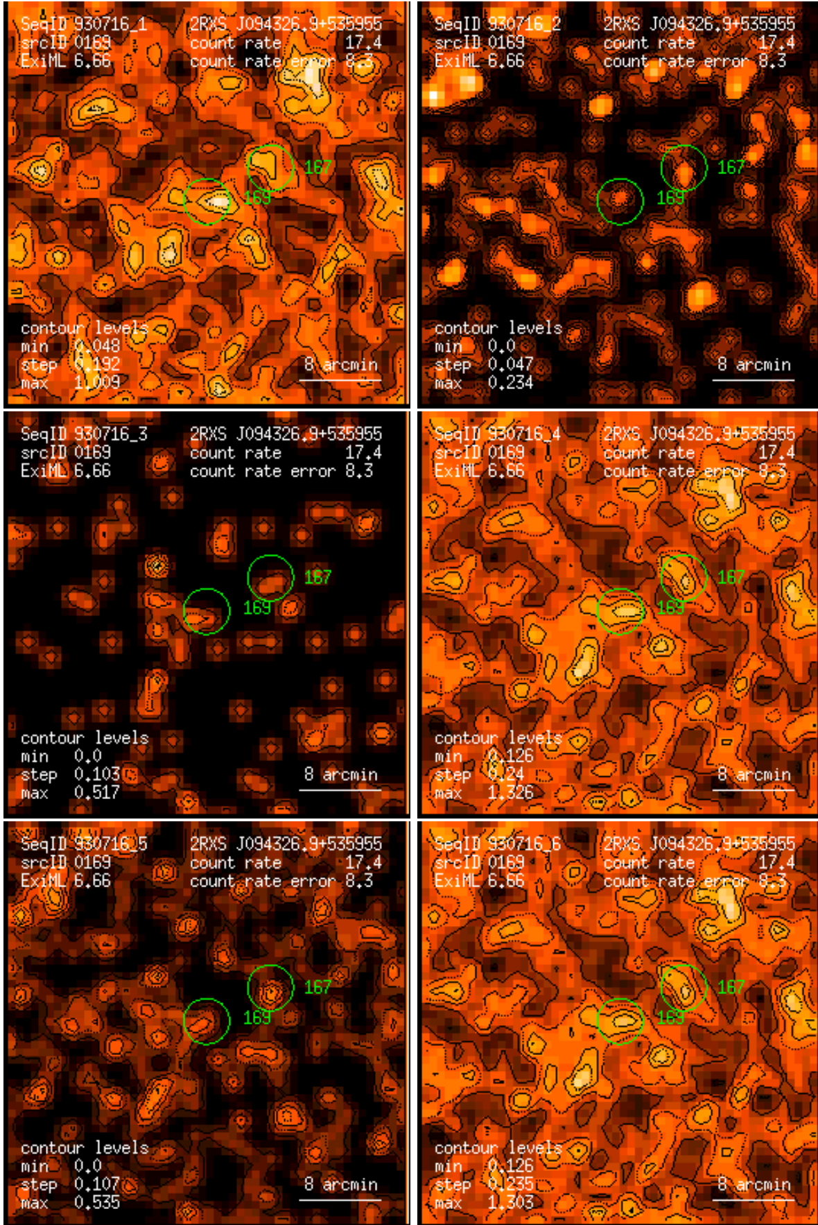
Figure 169: RASS 930716: detection 0169: band rate images, Gaussian filter: (1) PSPC channels 11 – 41, (2) 52 – 90, (3) 91 – 201, (4) 11 – 235, (5) 52 – 201, (6) 11 – 201. Broad band rates in counts/ks. Band rate contour levels in counts/ks/arcmin 2 .
