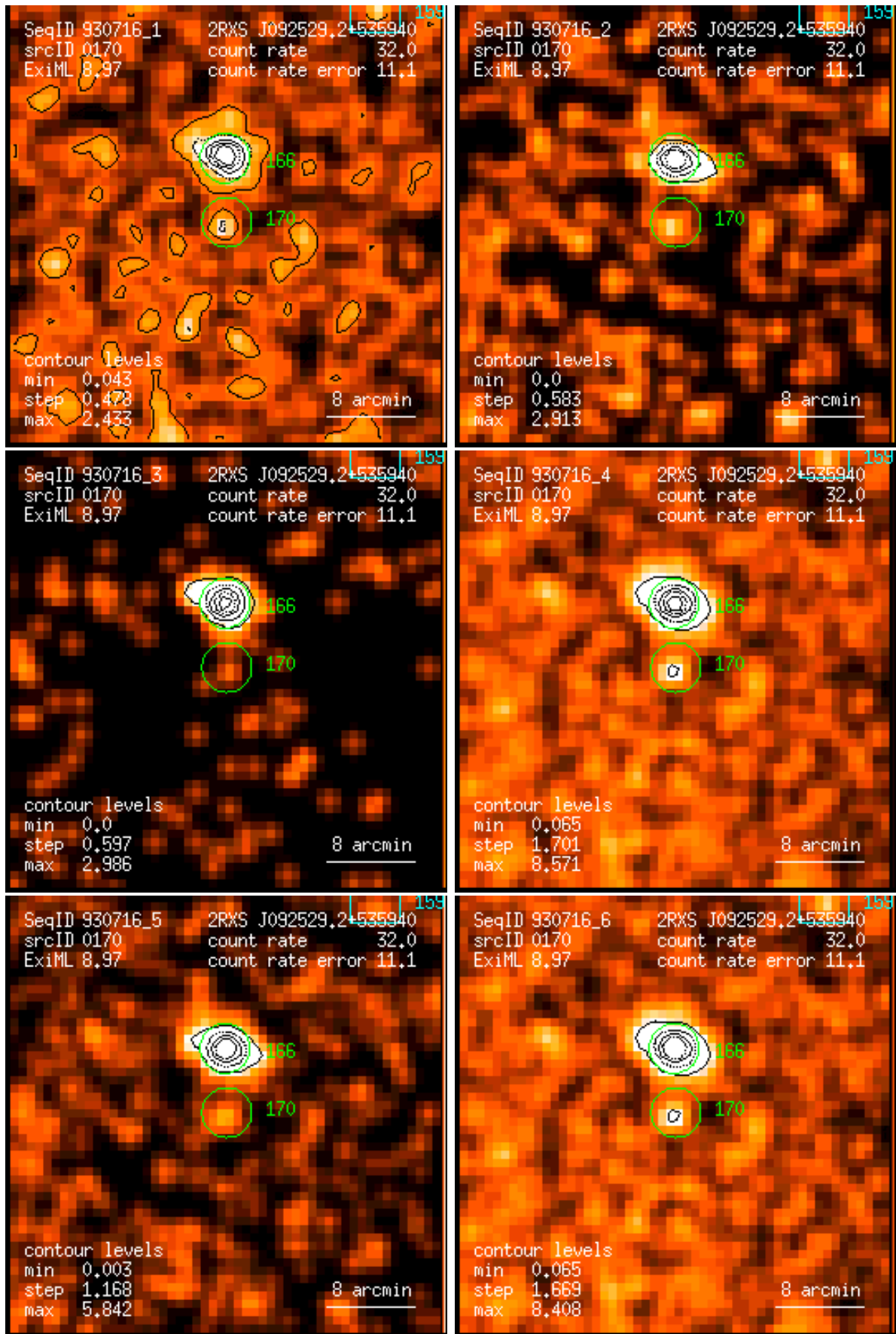
Figure 170: RASS 930716: detection 0170: band rate images, Gaussian filter: (1) PSPC channels 11 – 41, (2) 52 – 90, (3) 91 – 201, (4) 11 – 235, (5) 52 – 201, (6) 11 – 201. Broad band rates in counts/ks. Band rate contour levels in counts/ks/arcmin 2 .
