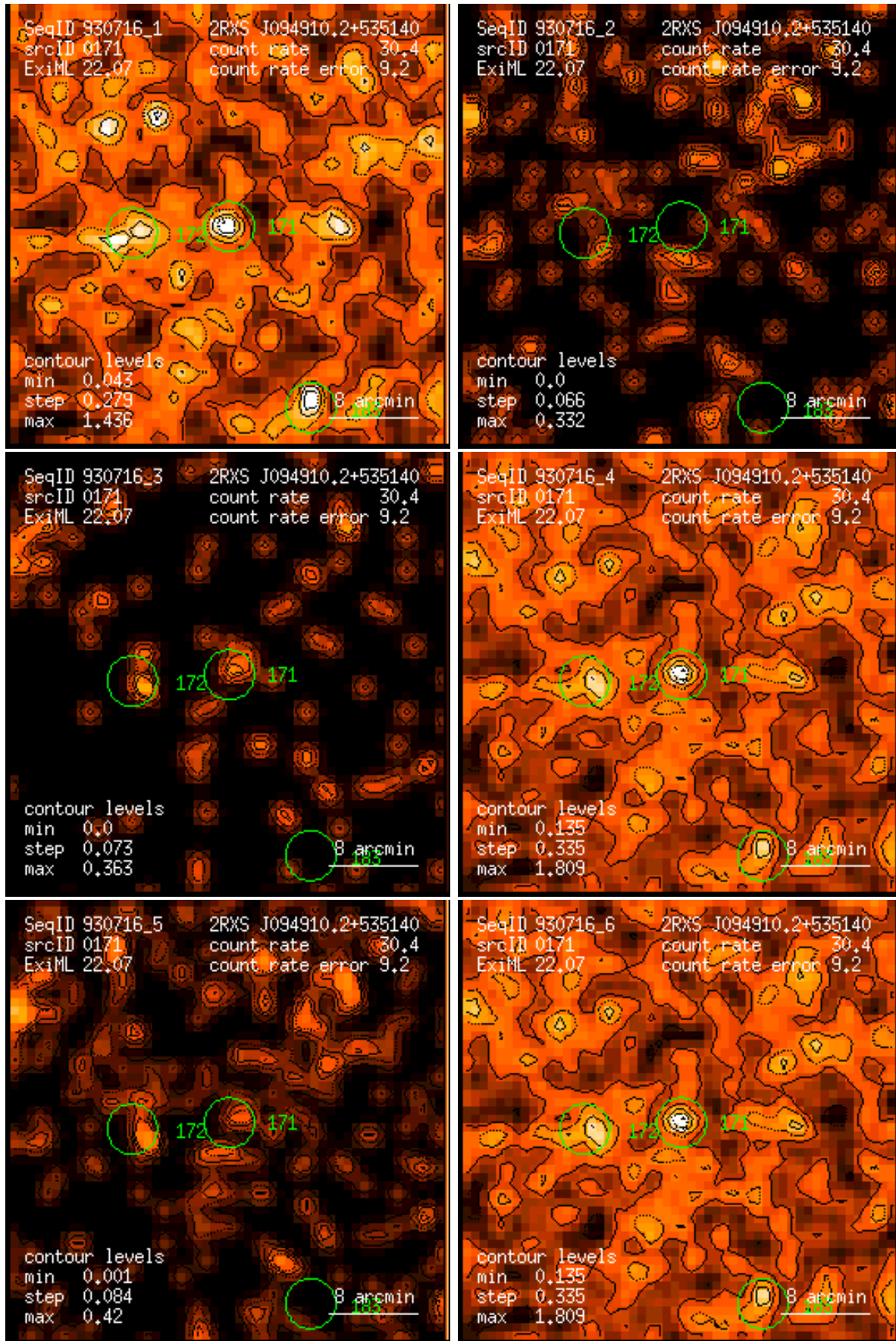
Figure 171: RASS 930716: detection 0171: band rate images, Gaussian filter: (1) PSPC channels 11 – 41, (2) 52 – 90, (3) 91 – 201, (4) 11 – 235, (5) 52 – 201, (6) 11 – 201. Broad band rates in counts/ks. Band rate contour levels in counts/ks/arcmin 2 .
