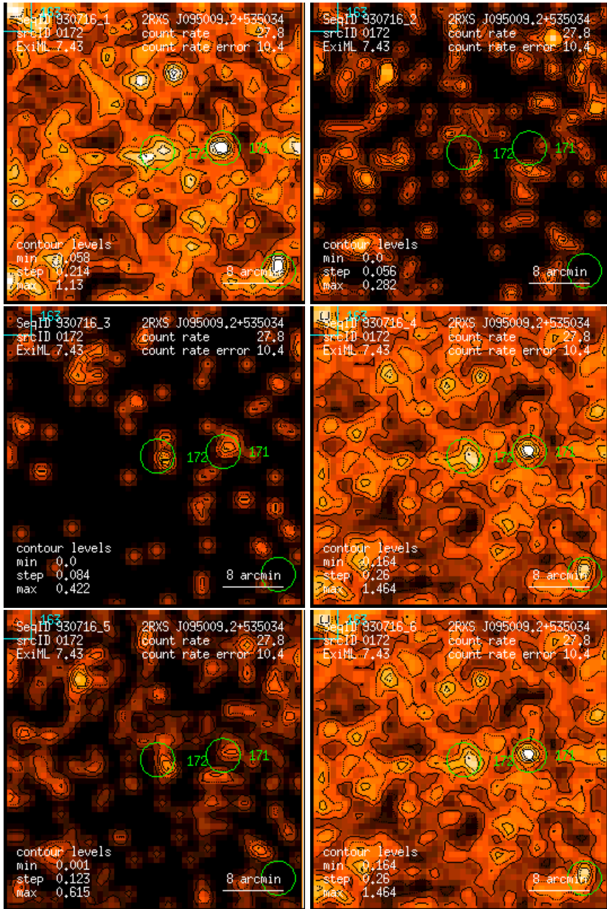
Figure 172: RASS 930716: detection 0172: band rate images, Gaussian filter: (1) PSPC channels 11 – 41, (2) 52 – 90, (3) 91 – 201, (4) 11 – 235, (5) 52 – 201, (6) 11 – 201. Broad band rates in counts/ks. Band rate contour levels in counts/ks/arcmin 2 .
