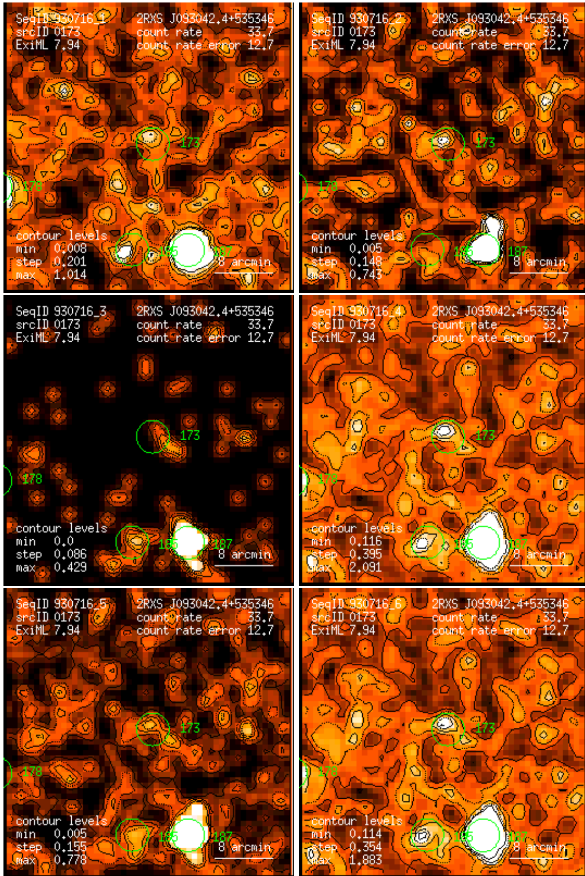
Figure 173: RASS 930716: detection 0173: band rate images, Gaussian filter: (1) PSPC channels 11 – 41, (2) 52 – 90, (3) 91 – 201, (4) 11 – 235, (5) 52 – 201, (6) 11 – 201. Broad band rates in counts/ks. Band rate contour levels in counts/ks/arcmin 2 .
