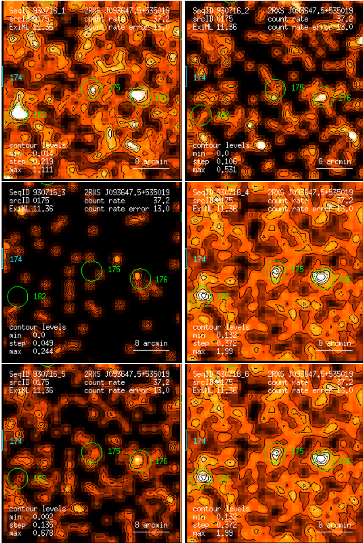
Figure 175: RASS 930716: detection 0175: band rate images, Gaussian filter: (1) PSPC channels 11 – 41, (2) 52 – 90, (3) 91 – 201, (4) 11 – 235, (5) 52 – 201, (6) 11 – 201. Broad band rates in counts/ks. Band rate contour levels in counts/ks/arcmin 2 .
