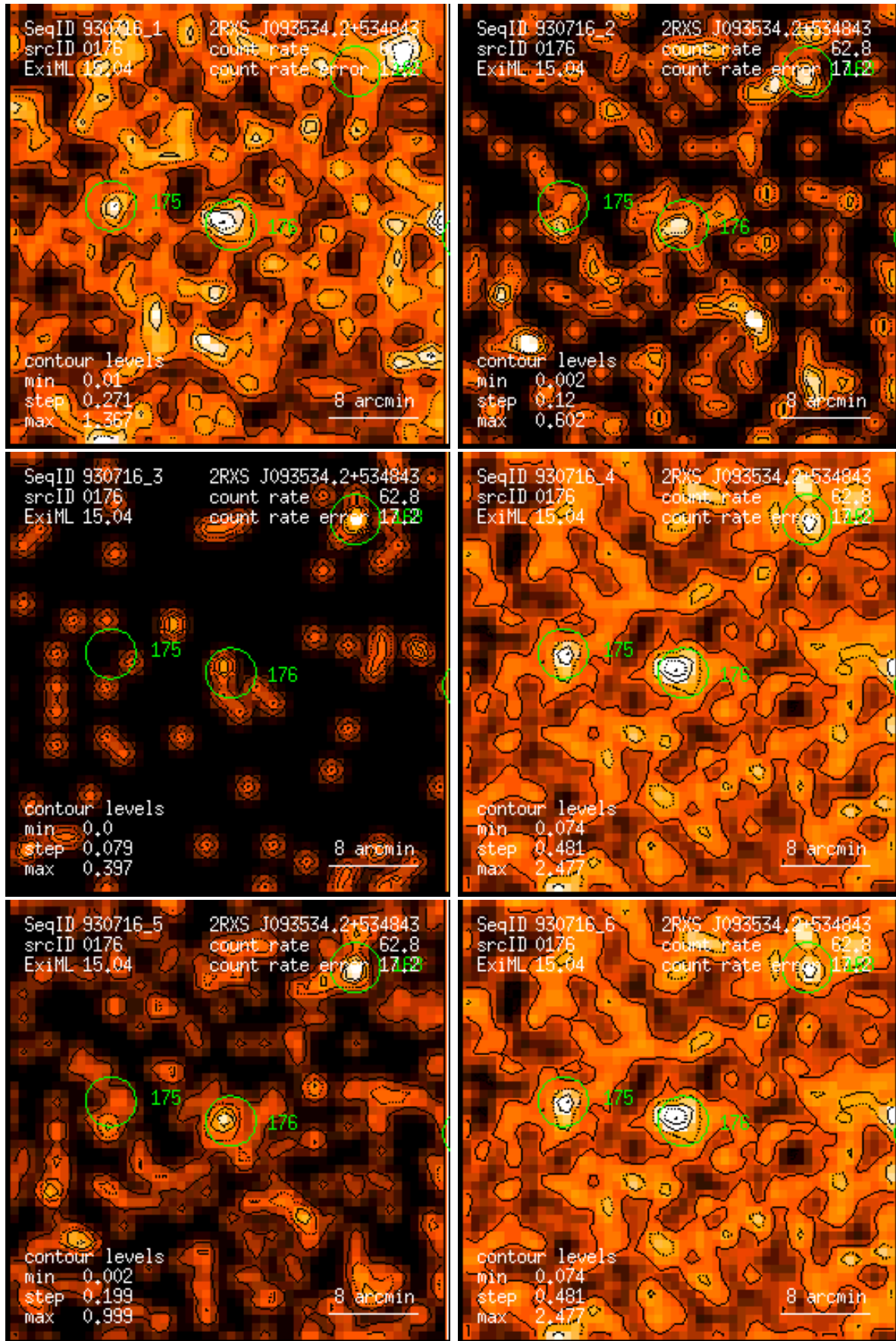
Figure 176: RASS 930716: detection 0176: band rate images, Gaussian filter: (1) PSPC channels 11 – 41, (2) 52 – 90, (3) 91 – 201, (4) 11 – 235, (5) 52 – 201, (6) 11 – 201. Broad band rates in counts/ks. Band rate contour levels in counts/ks/arcmin 2 .
