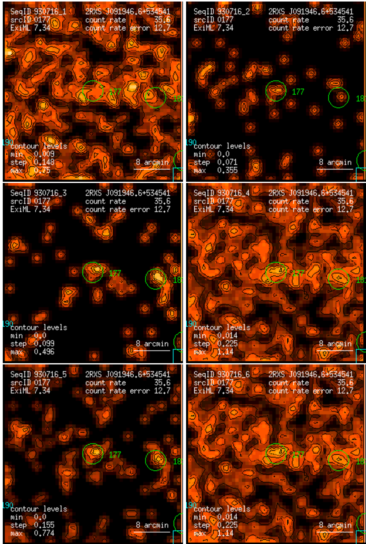
Figure 177: RASS 930716: detection 0177: band rate images, Gaussian filter: (1) PSPC channels 11 – 41, (2) 52 – 90, (3) 91 – 201, (4) 11 – 235, (5) 52 – 201, (6) 11 – 201. Broad band rates in counts/ks. Band rate contour levels in counts/ks/arcmin 2 .
