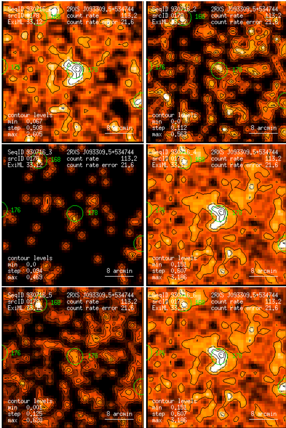
Figure 178: RASS 930716: detection 0178: band rate images, Gaussian filter: (1) PSPC channels 11 – 41, (2) 52 – 90, (3) 91 – 201, (4) 11 – 235, (5) 52 – 201, (6) 11 – 201. Broad band rates in counts/ks. Band rate contour levels in counts/ks/arcmin 2 .
