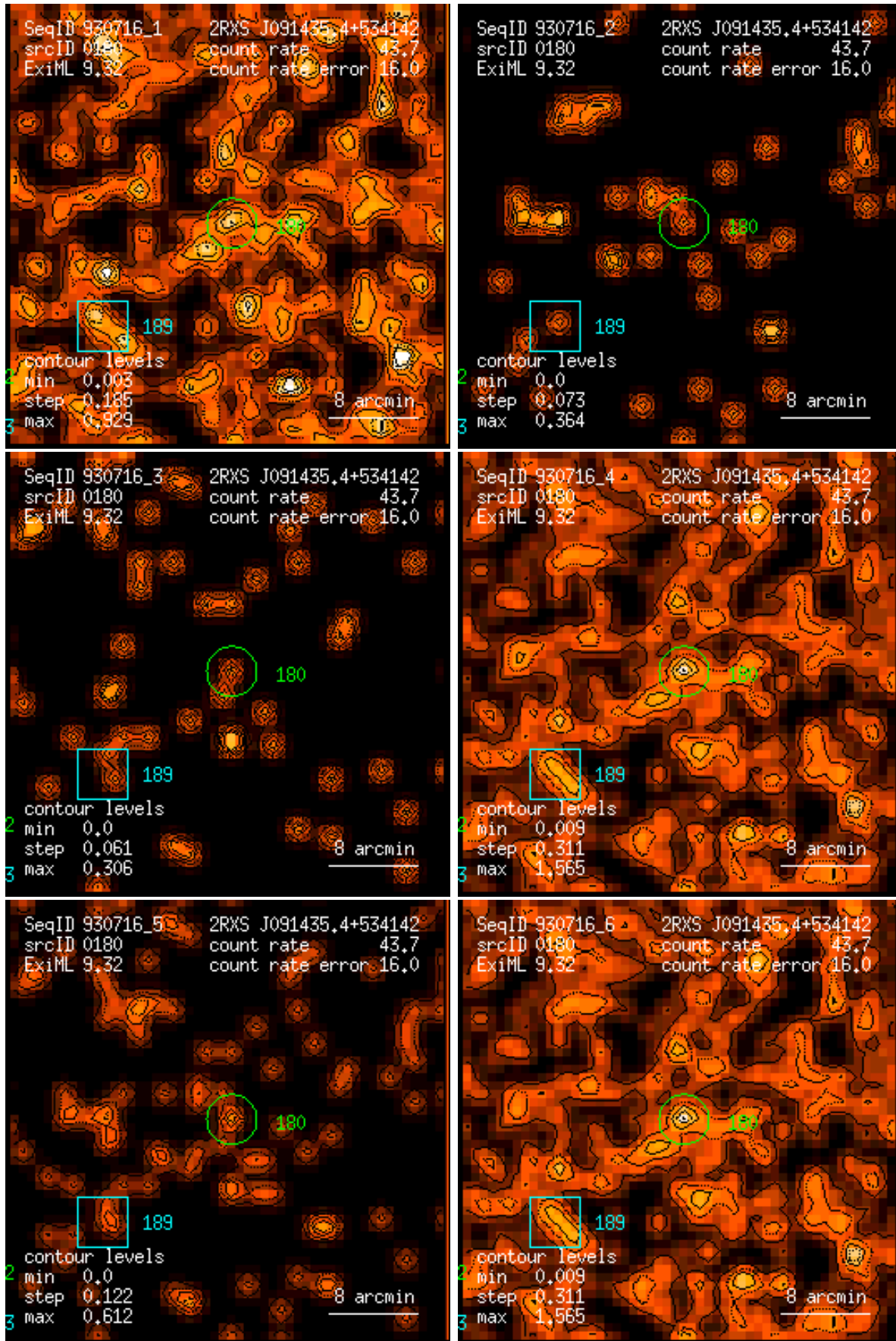
Figure 180: RASS 930716: detection 0180: band rate images, Gaussian filter: (1) PSPC channels 11 – 41, (2) 52 – 90, (3) 91 – 201, (4) 11 – 235, (5) 52 – 201, (6) 11 – 201. Broad band rates in counts/ks. Band rate contour levels in counts/ks/arcmin 2 .
