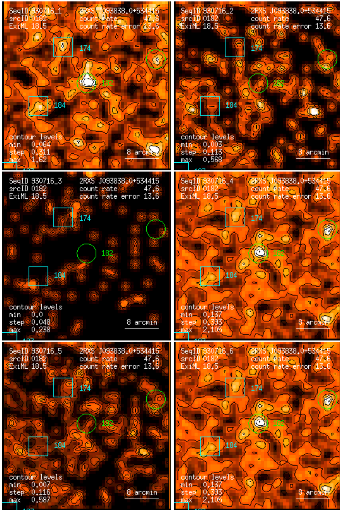
Figure 182: RASS 930716: detection 0182: band rate images, Gaussian filter: (1) PSPC channels 11 – 41, (2) 52 – 90, (3) 91 – 201, (4) 11 – 235, (5) 52 – 201, (6) 11 – 201. Broad band rates in counts/ks. Band rate contour levels in counts/ks/arcmin 2 .
