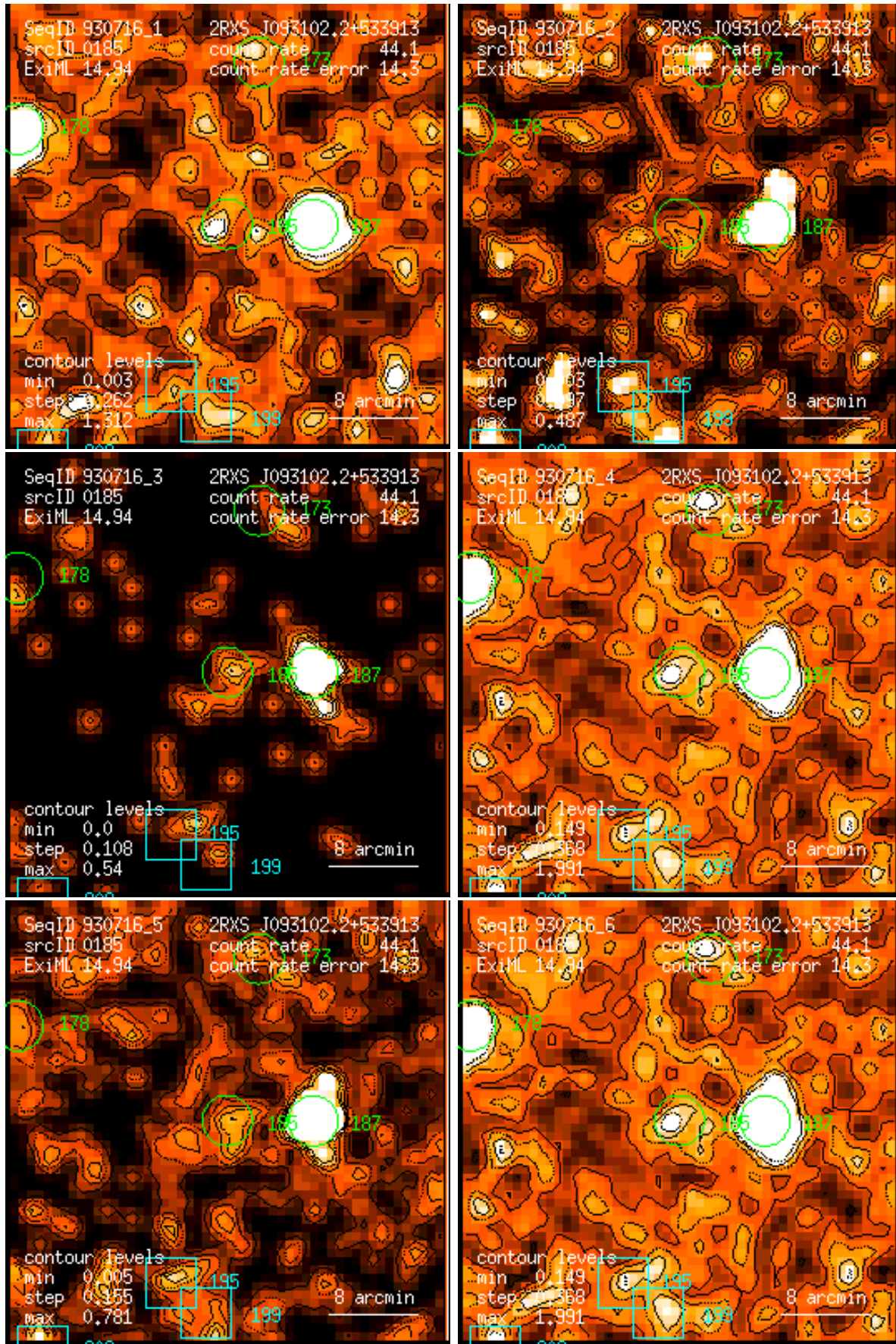
Figure 185: RASS 930716: detection 0185: band rate images, Gaussian filter: (1) PSPC channels 11 – 41, (2) 52 – 90, (3) 91 – 201, (4) 11 – 235, (5) 52 – 201, (6) 11 – 201. Broad band rates in counts/ks. Band rate contour levels in counts/ks/arcmin 2 .
