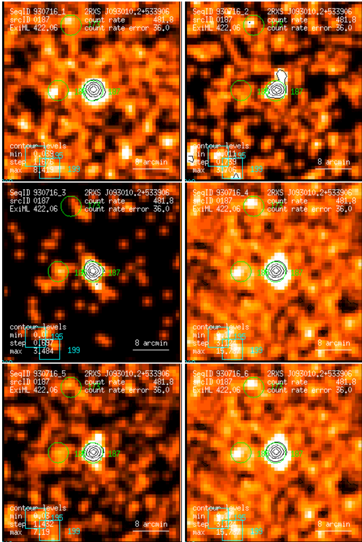
Figure 187: RASS 930716: detection 0187: band rate images, Gaussian filter: (1) PSPC channels 11 – 41, (2) 52 – 90, (3) 91 – 201, (4) 11 – 235, (5) 52 – 201, (6) 11 – 201. Broad band rates in counts/ks. Band rate contour levels in counts/ks/arcmin 2 .
