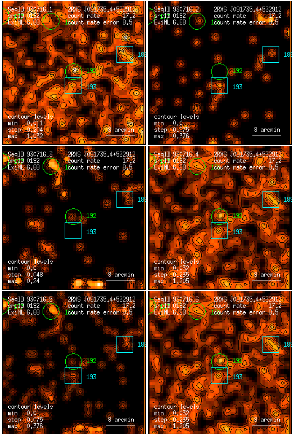
Figure 192: RASS 930716: detection 0192: band rate images, Gaussian filter: (1) PSPC channels 11 – 41, (2) 52 – 90, (3) 91 – 201, (4) 11 – 235, (5) 52 – 201, (6) 11 – 201. Broad band rates in counts/ks. Band rate contour levels in counts/ks/arcmin 2 .
