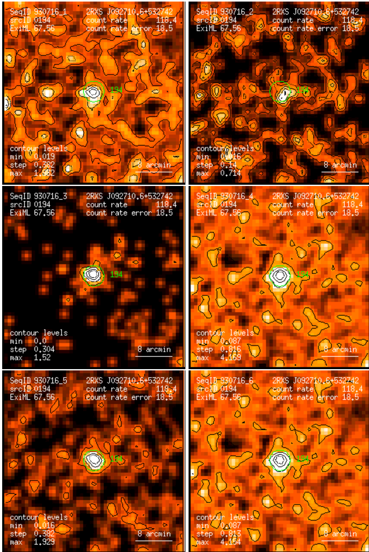
Figure 194: RASS 930716: detection 0194: band rate images, Gaussian filter: (1) PSPC channels 11 – 41, (2) 52 – 90, (3) 91 – 201, (4) 11 – 235, (5) 52 – 201, (6) 11 – 201. Broad band rates in counts/ks. Band rate contour levels in counts/ks/arcmin 2 .
